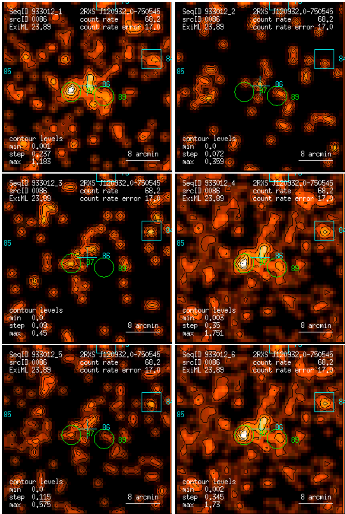
Figure 86: RASS 933012: detection 0086: band rate images, Gaussian filter: (1) PSPC channels 11 – 41, (2) 52 – 90, (3) 91 – 201, (4) 11 – 235, (5) 52 – 201, (6) 11 – 201. Broad band rates in counts/ks. Band rate contour levels in counts/ks/arcmin 2 .
