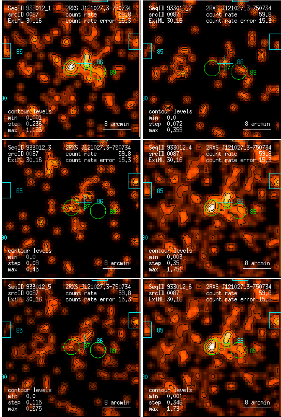
Figure 87: RASS 933012: detection 0087: band rate images, Gaussian filter: (1) PSPC channels 11 – 41, (2) 52 – 90, (3) 91 – 201, (4) 11 – 235, (5) 52 – 201, (6) 11 – 201. Broad band rates in counts/ks. Band rate contour levels in counts/ks/arcmin 2 .
