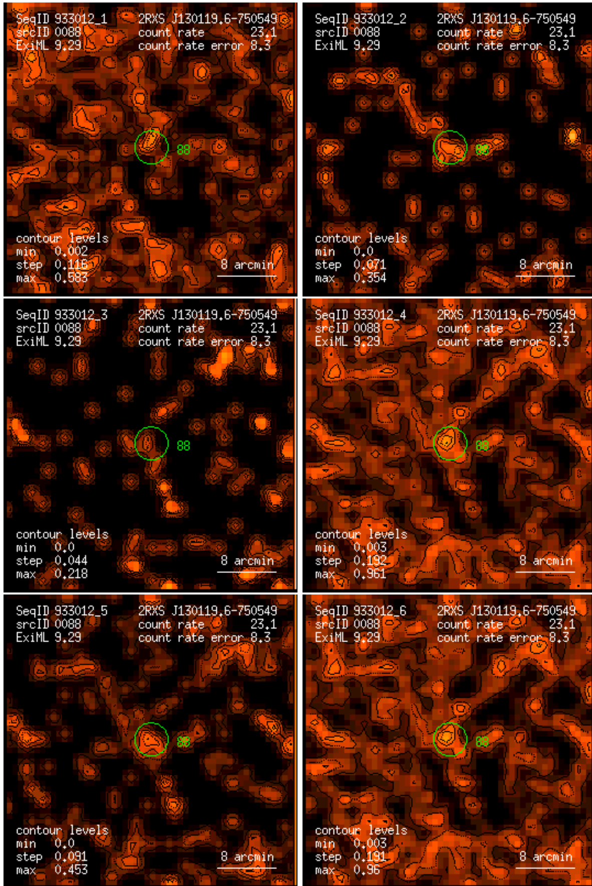
Figure 88: RASS 933012: detection 0088: band rate images, Gaussian filter: (1) PSPC channels 11 – 41, (2) 52 – 90, (3) 91 – 201, (4) 11 – 235, (5) 52 – 201, (6) 11 – 201. Broad band rates in counts/ks. Band rate contour levels in counts/ks/arcmin 2 .
