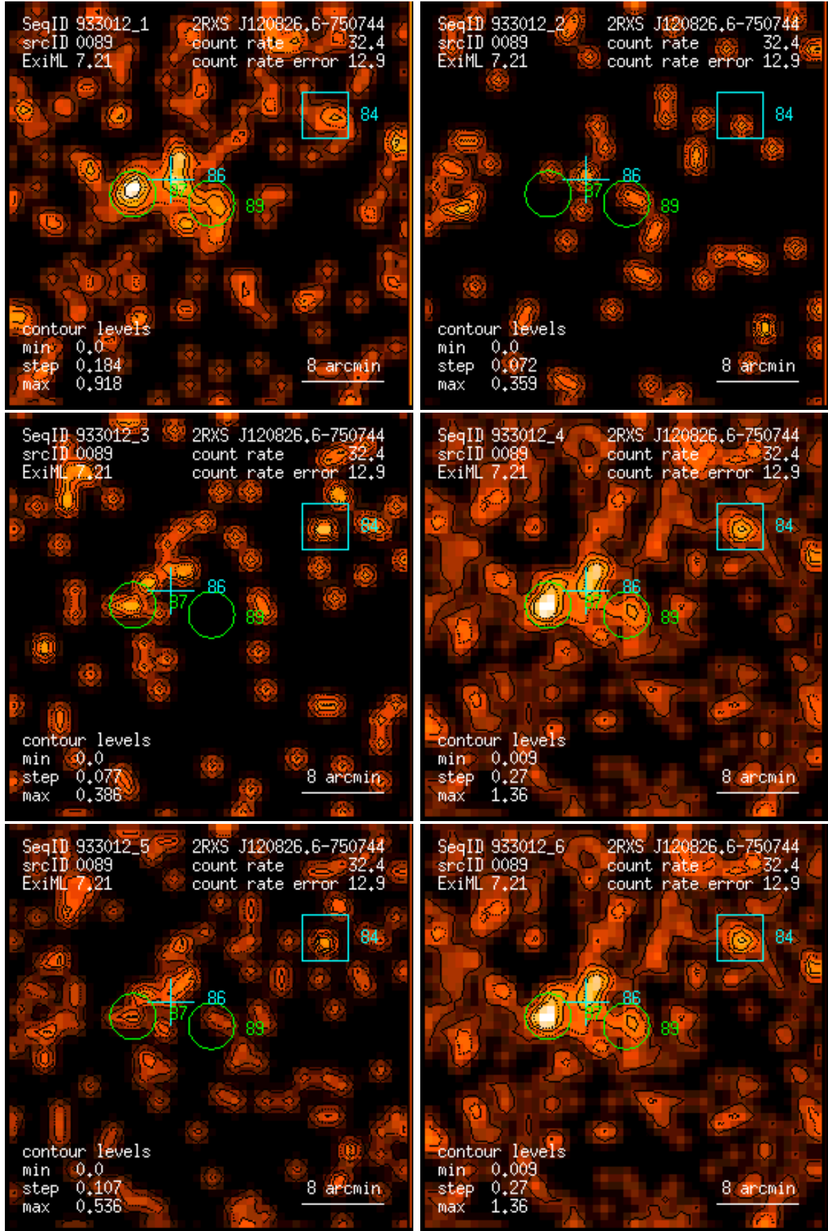
Figure 89: RASS 933012: detection 0089: band rate images, Gaussian filter: (1) PSPC channels 11 – 41, (2) 52 – 90, (3) 91 – 201, (4) 11 – 235, (5) 52 – 201, (6) 11 – 201. Broad band rates in counts/ks. Band rate contour levels in counts/ks/arcmin 2 .
