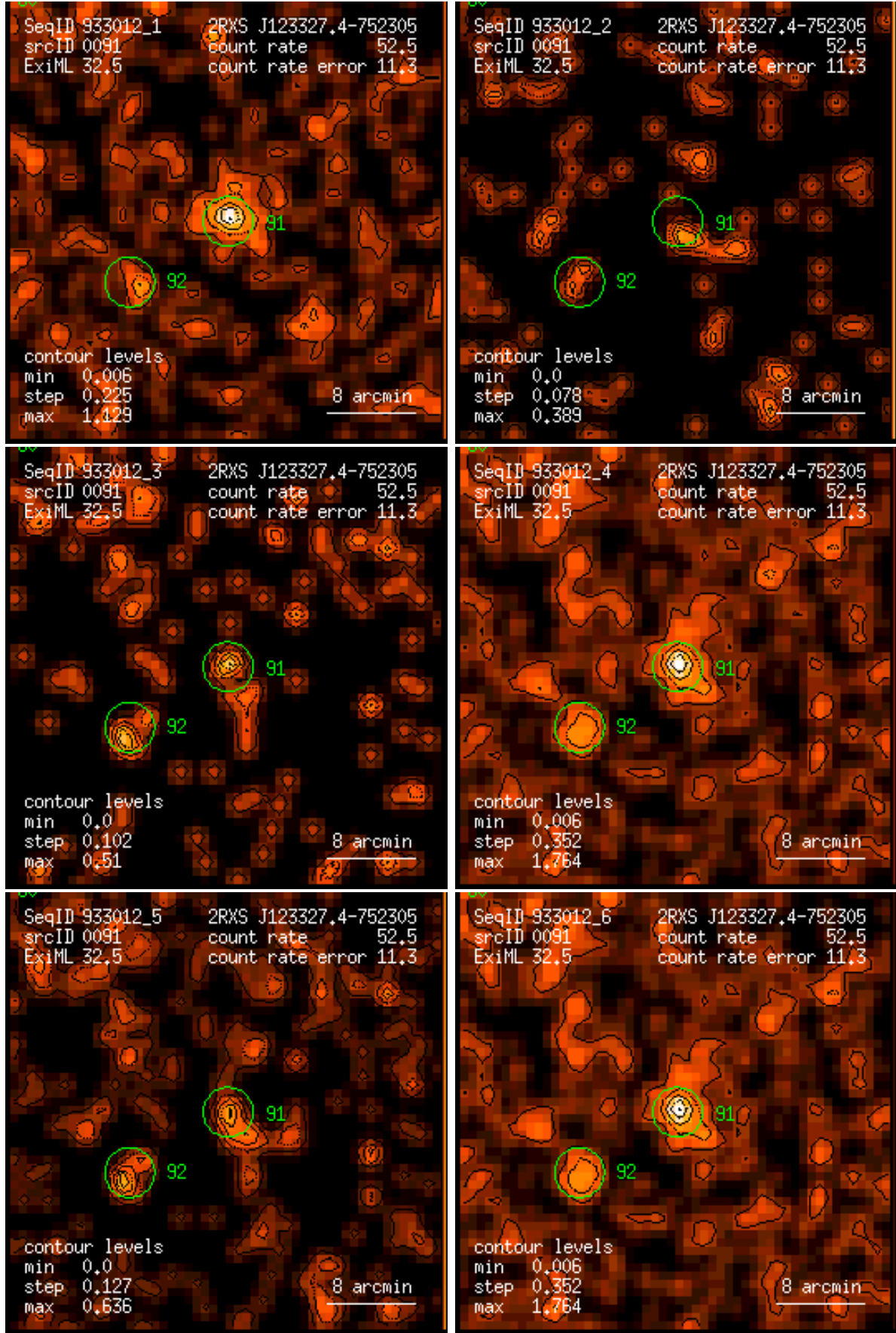
Figure 91: RASS 933012: detection 0091: band rate images, Gaussian filter: (1) PSPC channels 11 – 41, (2) 52 – 90, (3) 91 – 201, (4) 11 – 235, (5) 52 – 201, (6) 11 – 201. Broad band rates in counts/ks. Band rate contour levels in counts/ks/arcmin 2 .
