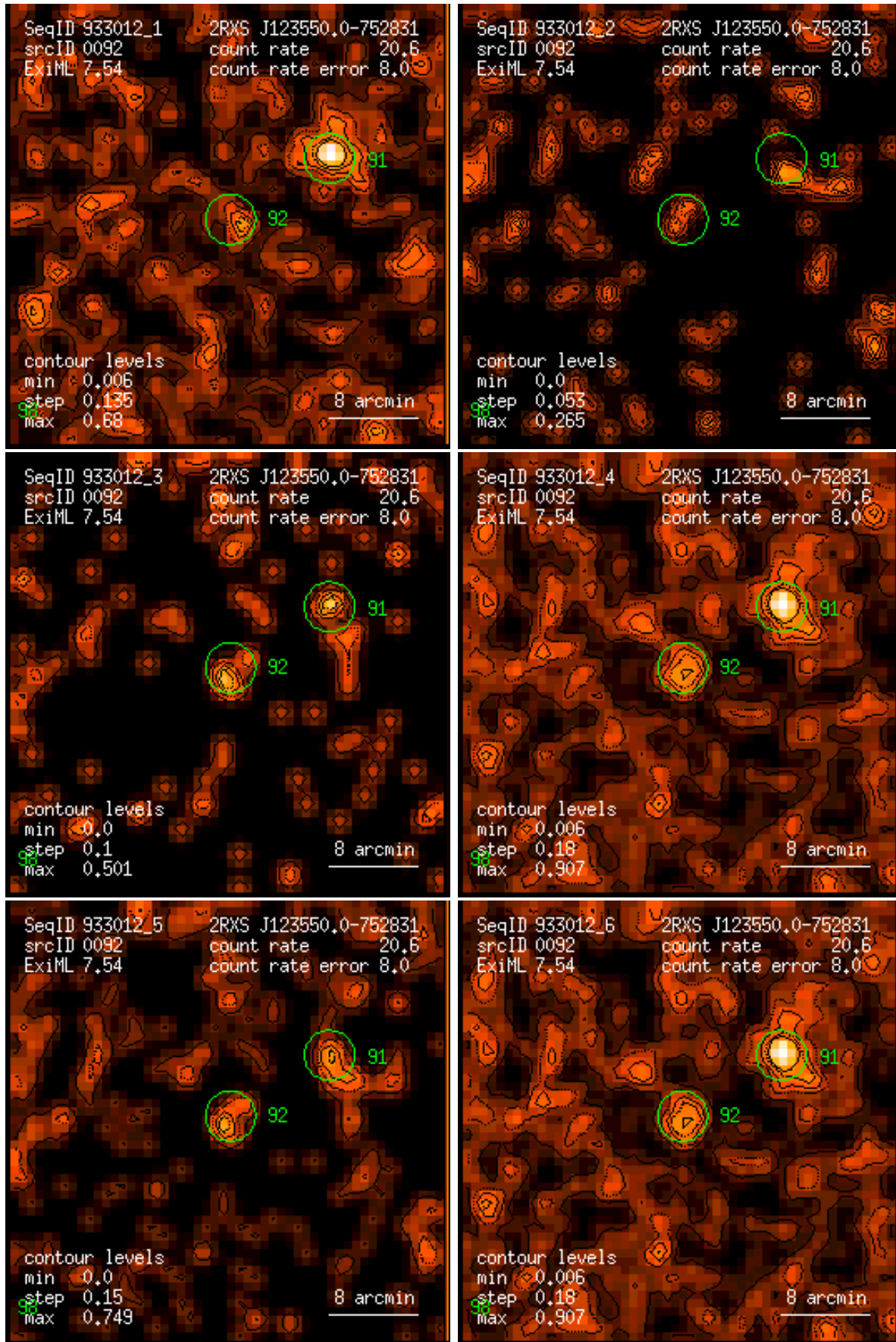
Figure 92: RASS 933012: detection 0092: band rate images, Gaussian filter: (1) PSPC channels 11 – 41, (2) 52 – 90, (3) 91 – 201, (4) 11 – 235, (5) 52 – 201, (6) 11 – 201. Broad band rates in counts/ks. Band rate contour levels in counts/ks/arcmin 2 .
