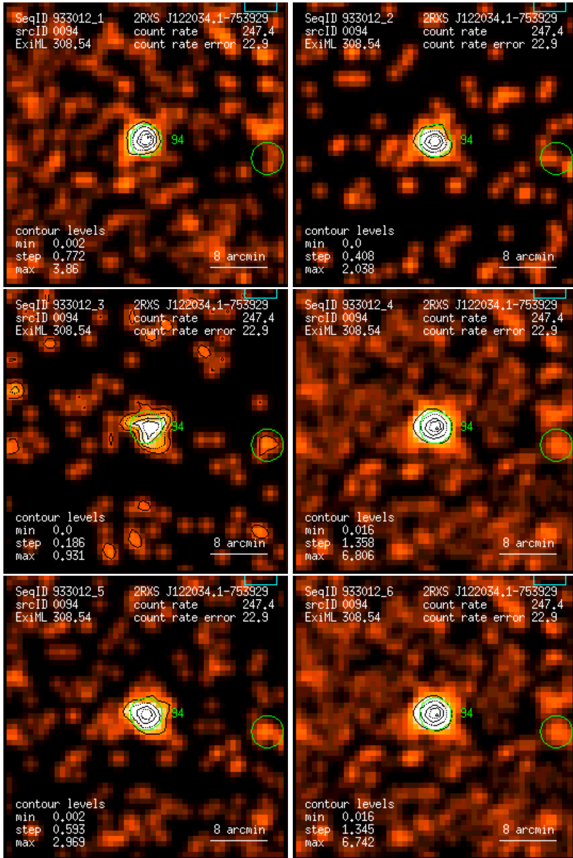
Figure 94: RASS 933012: detection 0094: band rate images, Gaussian filter: (1) PSPC channels 11 – 41, (2) 52 – 90, (3) 91 – 201, (4) 11 – 235, (5) 52 – 201, (6) 11 – 201. Broad band rates in counts/ks. Band rate contour levels in counts/ks/arcmin 2 .
