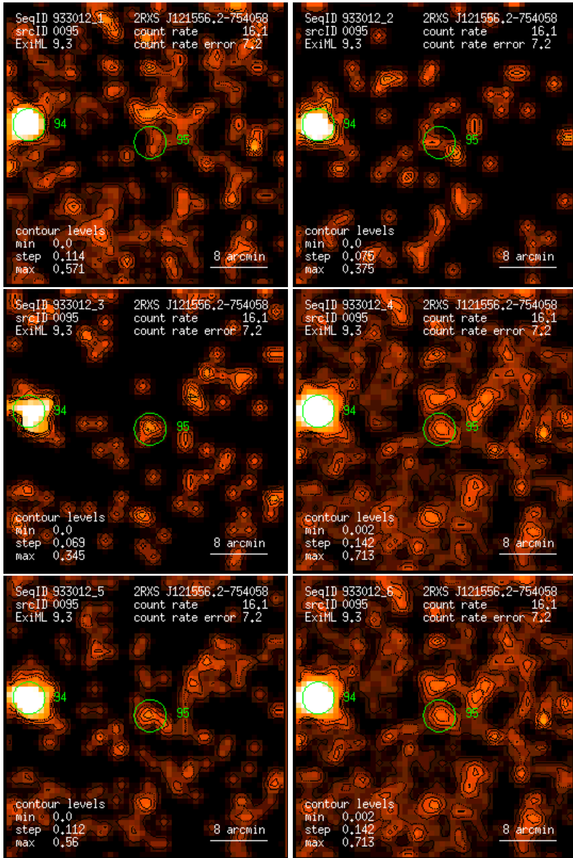
Figure 95: RASS 933012: detection 0095: band rate images, Gaussian filter: (1) PSPC channels 11 – 41, (2) 52 – 90, (3) 91 – 201, (4) 11 – 235, (5) 52 – 201, (6) 11 – 201. Broad band rates in counts/ks. Band rate contour levels in counts/ks/arcmin 2 .
