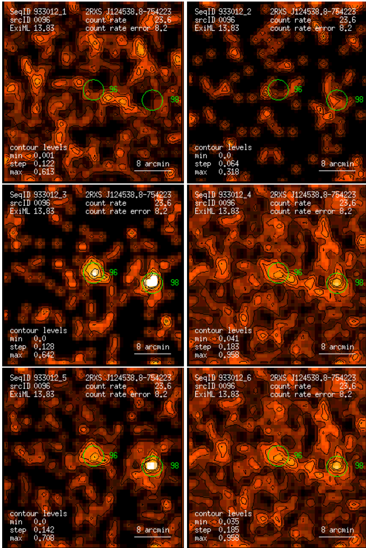
Figure 96: RASS 933012: detection 0096: band rate images, Gaussian filter: (1) PSPC channels 11 – 41, (2) 52 – 90, (3) 91 – 201, (4) 11 – 235, (5) 52 – 201, (6) 11 – 201. Broad band rates in counts/ks. Band rate contour levels in counts/ks/arcmin 2 .
