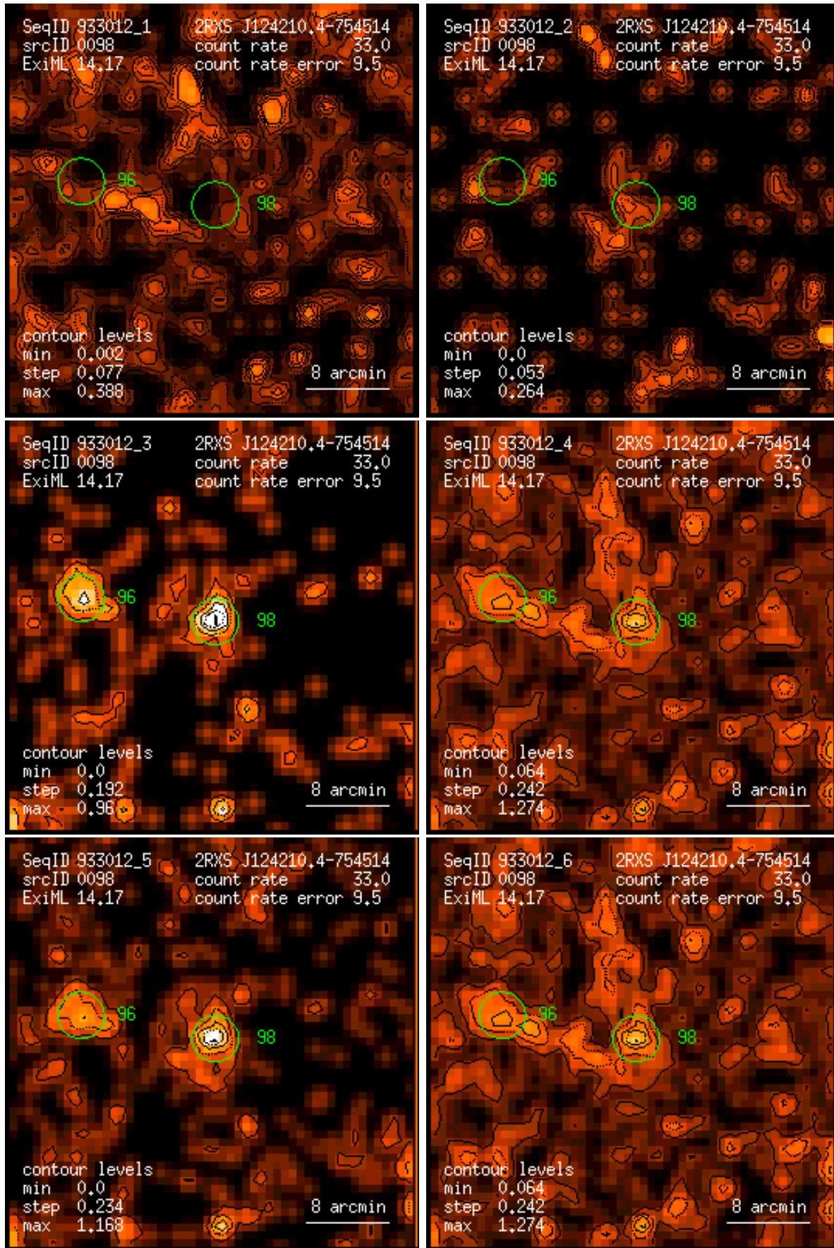
Figure 98: RASS 933012: detection 0098: band rate images, Gaussian filter: (1) PSPC channels 11 – 41, (2) 52 – 90, (3) 91 – 201, (4) 11 – 235, (5) 52 – 201, (6) 11 – 201. Broad band rates in counts/ks. Band rate contour levels in counts/ks/arcmin 2 .
