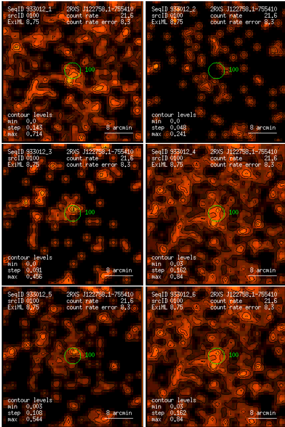
Figure 100: RASS 933012: detection 0100: band rate images, Gaussian filter: (1) PSPC channels 11 – 41, (2) 52 – 90, (3) 91 – 201, (4) 11 – 235, (5) 52 – 201, (6) 11 – 201. Broad band rates in counts/ks. Band rate contour levels in counts/ks/arcmin 2 .
