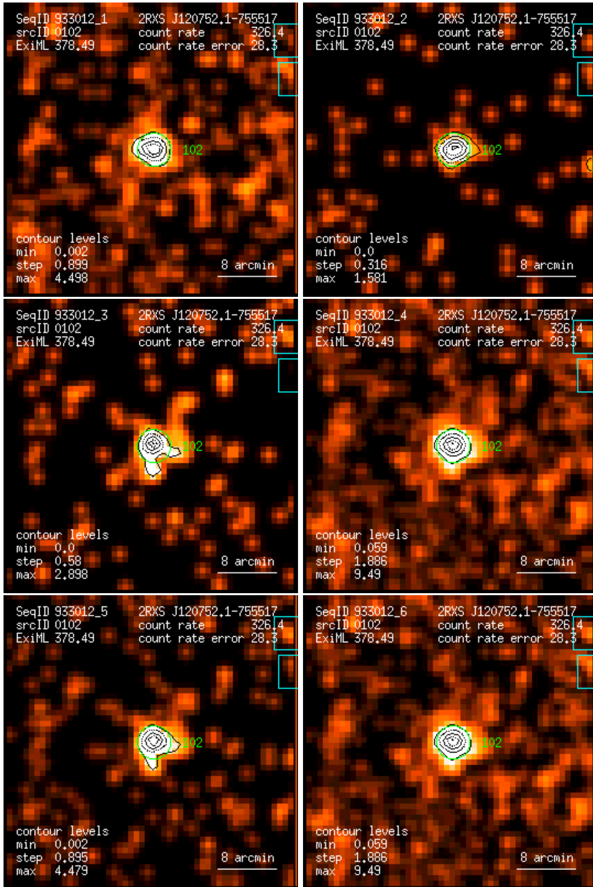
Figure 102: RASS 933012: detection 0102: band rate images, Gaussian filter: (1) PSPC channels 11 – 41, (2) 52 – 90, (3) 91 – 201, (4) 11 – 235, (5) 52 – 201, (6) 11 – 201. Broad band rates in counts/ks. Band rate contour levels in counts/ks/arcmin 2 .
