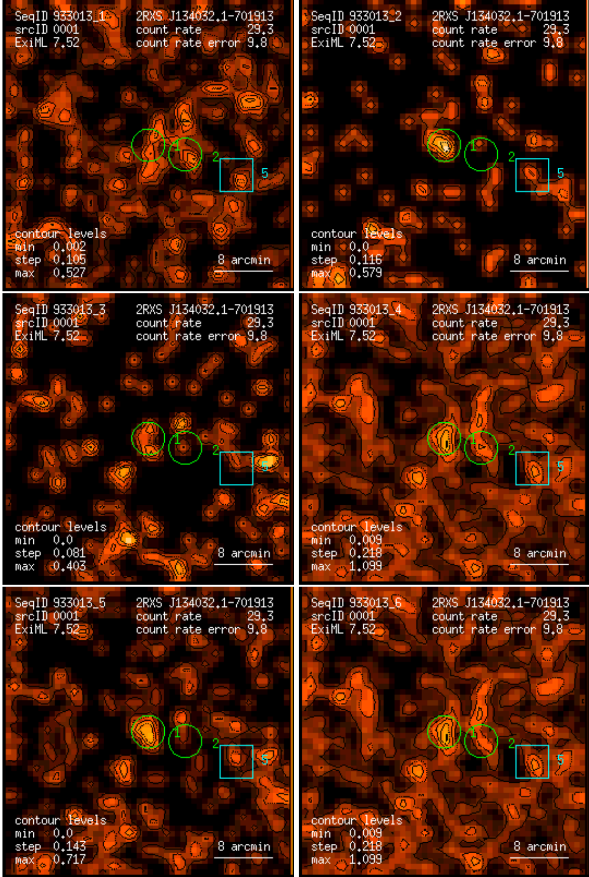
Figure 1: RASS 933013: detection 0001: band rate images, Gaussian filter: (1) PSPC channels 11 – 41, (2) 52 – 90, (3) 91 – 201, (4) 11 – 235, (5) 52 – 201, (6) 11 – 201. Broad band rates in counts/ks. Band rate contour levels in counts/ks/arcmin 2 .
