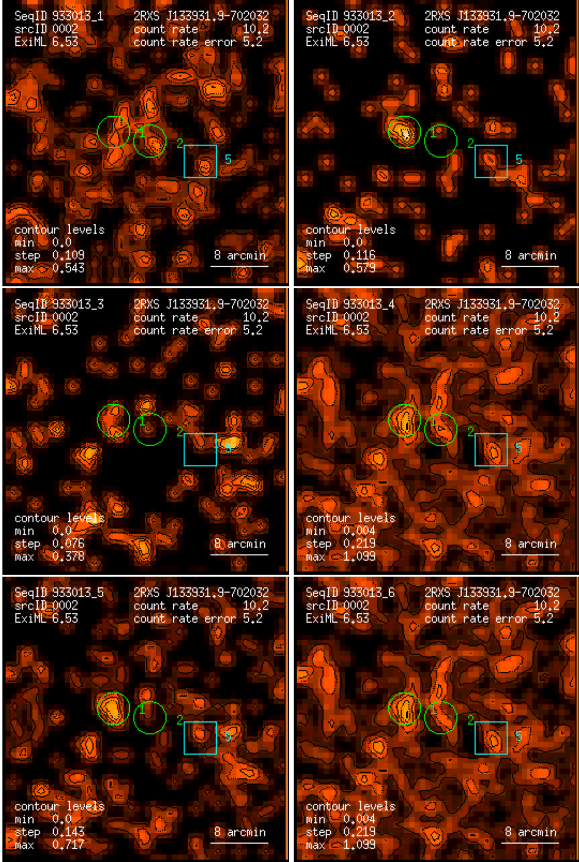
Figure 2: RASS 933013: detection 0002: band rate images, Gaussian filter: (1) PSPC channels 11 – 41, (2) 52 – 90, (3) 91 – 201, (4) 11 – 235, (5) 52 – 201, (6) 11 – 201. Broad band rates in counts/ks. Band rate contour levels in counts/ks/arcmin 2 .
