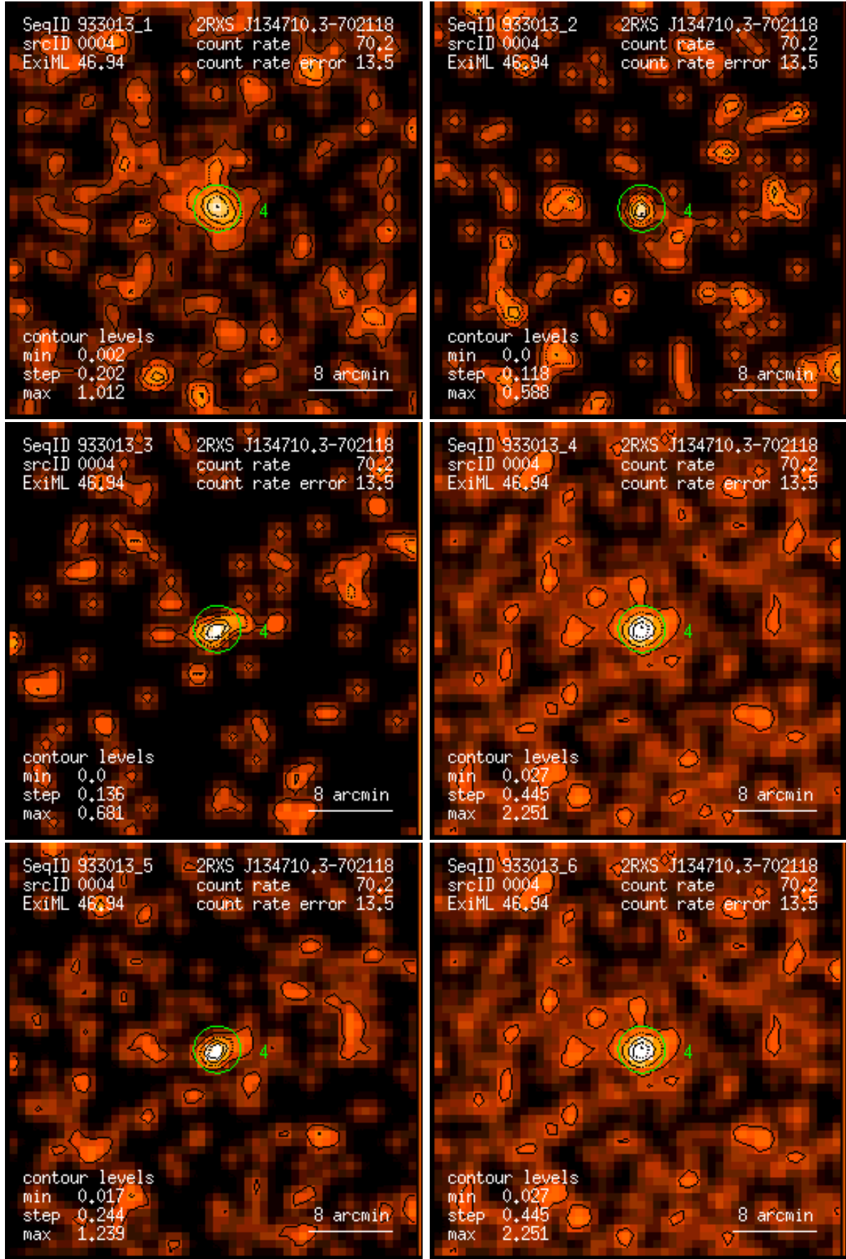
Figure 4: RASS 933013: detection 0004: band rate images, Gaussian filter: (1) PSPC channels 11 – 41, (2) 52 – 90, (3) 91 – 201, (4) 11 – 235, (5) 52 – 201, (6) 11 – 201. Broad band rates in counts/ks. Band rate contour levels in counts/ks/arcmin 2 .
