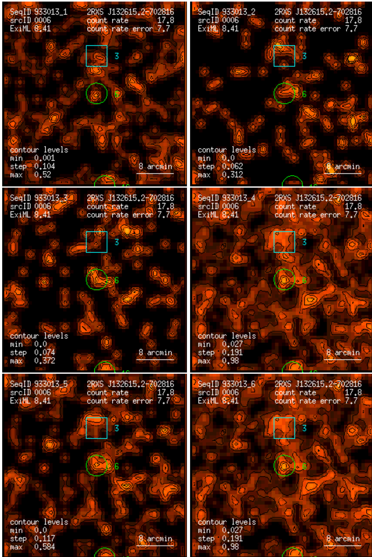
Figure 6: RASS 933013: detection 0006: band rate images, Gaussian filter: (1) PSPC channels 11 – 41, (2) 52 – 90, (3) 91 – 201, (4) 11 – 235, (5) 52 – 201, (6) 11 – 201. Broad band rates in counts/ks. Band rate contour levels in counts/ks/arcmin 2 .
