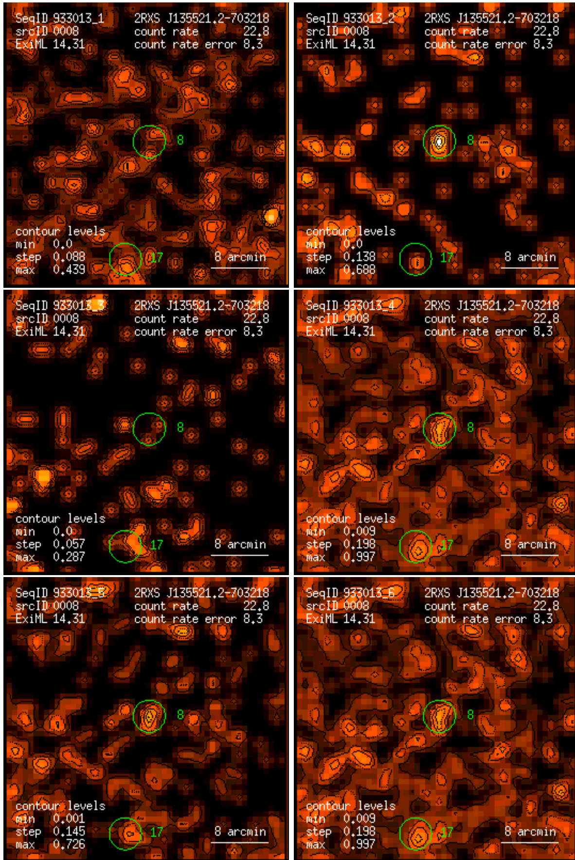
Figure 8: RASS 933013: detection 0008: band rate images, Gaussian filter: (1) PSPC channels 11 – 41, (2) 52 – 90, (3) 91 – 201, (4) 11 – 235, (5) 52 – 201, (6) 11 – 201. Broad band rates in counts/ks. Band rate contour levels in counts/ks/arcmin 2 .
