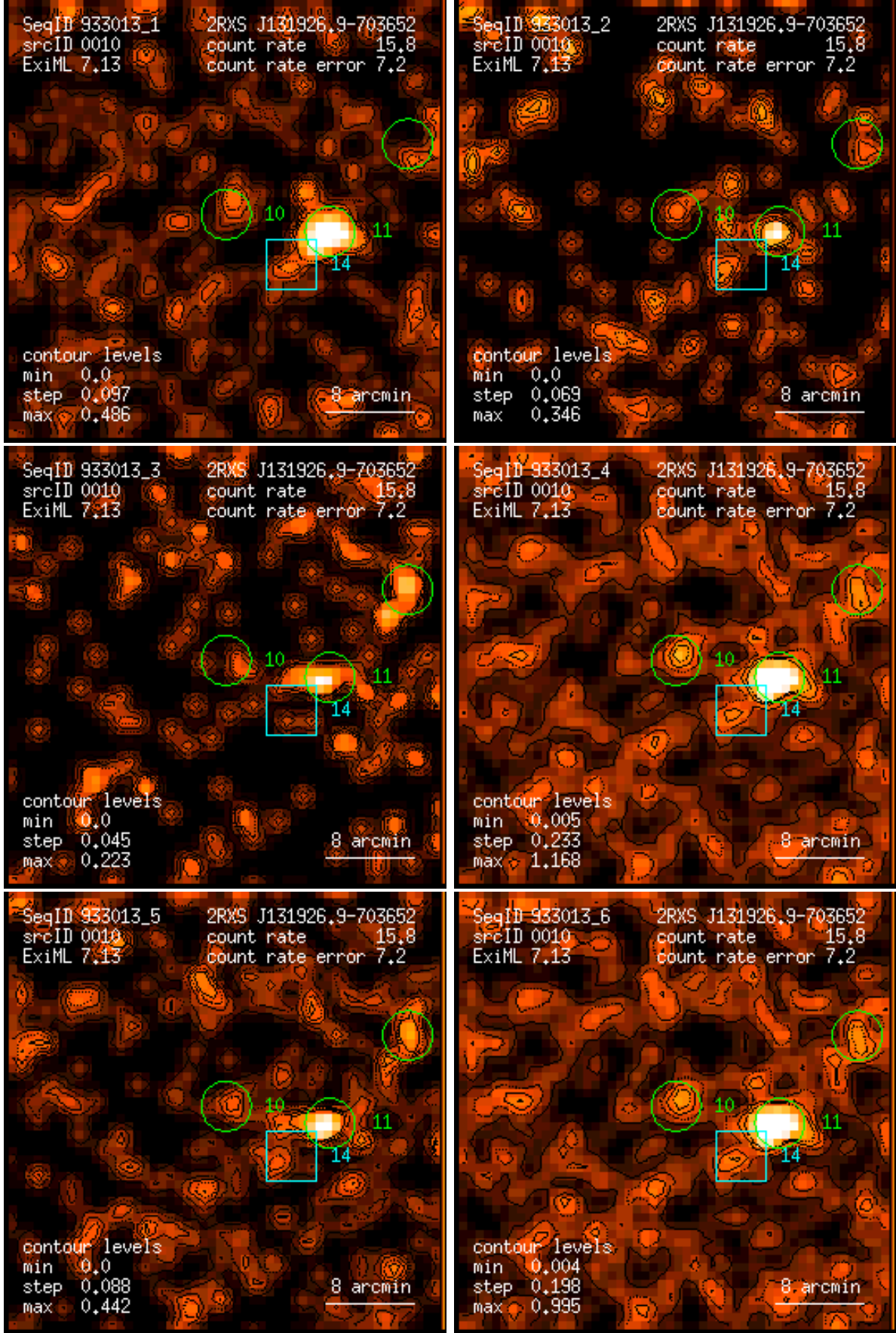
Figure 10: RASS 933013: detection 0010: band rate images, Gaussian filter: (1) PSPC channels 11 – 41, (2) 52 – 90, (3) 91 – 201, (4) 11 – 235, (5) 52 – 201, (6) 11 – 201. Broad band rates in counts/ks. Band rate contour levels in counts/ks/arcmin 2 .
