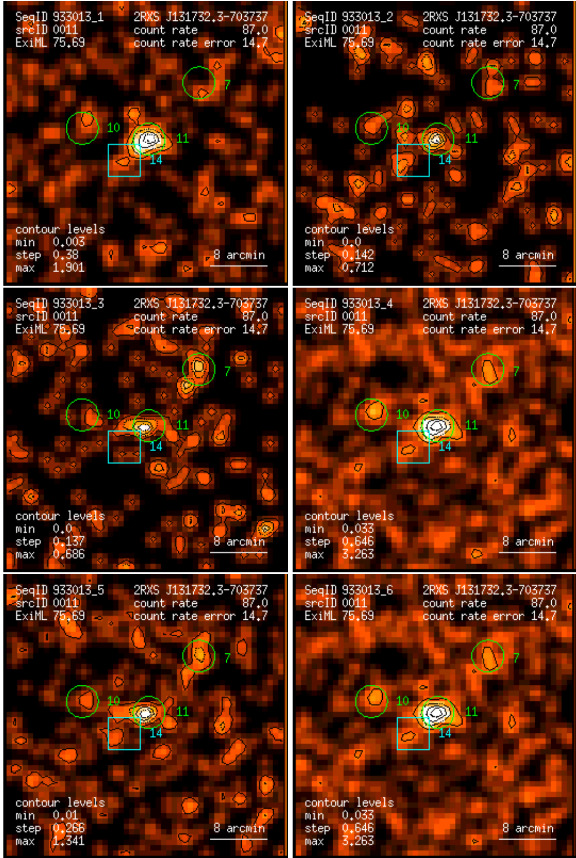
Figure 11: RASS 933013: detection 0011: band rate images, Gaussian filter: (1) PSPC channels 11 – 41, (2) 52 – 90, (3) 91 – 201, (4) 11 – 235, (5) 52 – 201, (6) 11 – 201. Broad band rates in counts/ks. Band rate contour levels in counts/ks/arcmin 2 .
