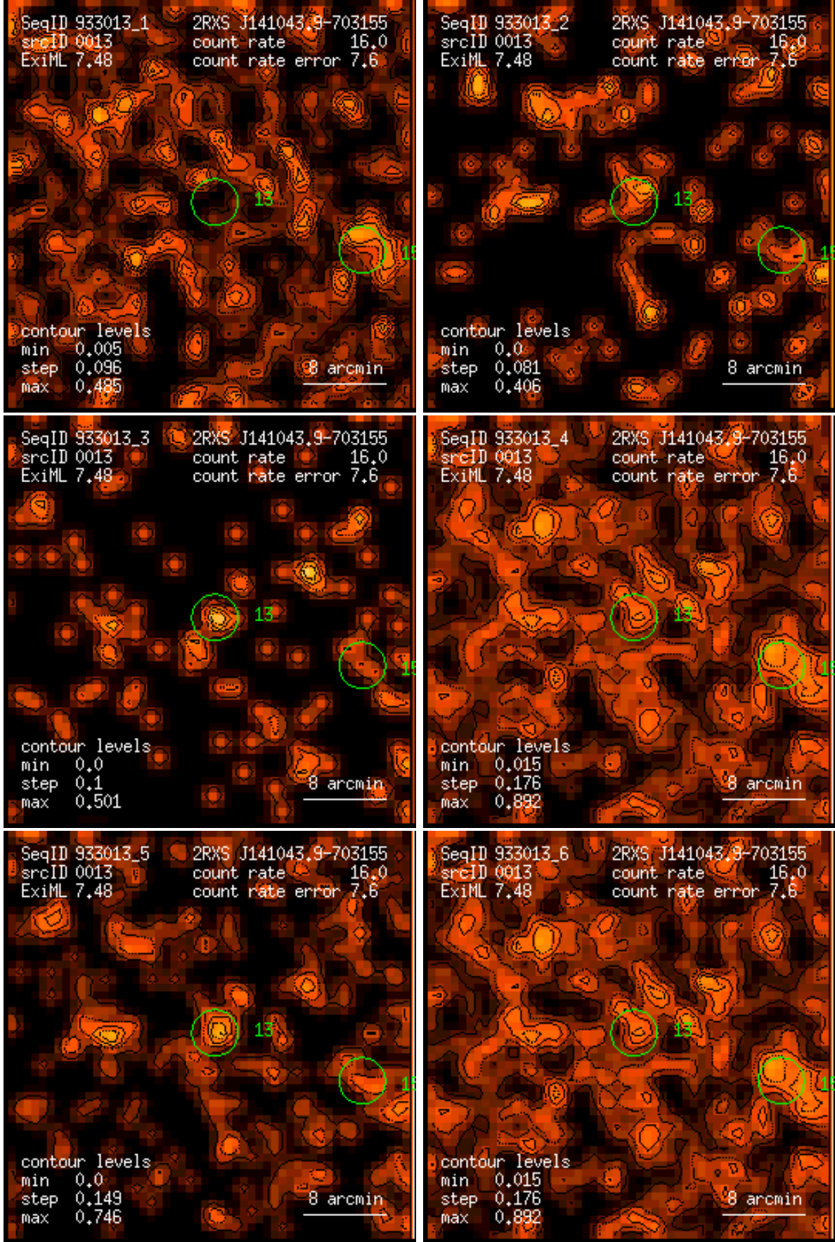
Figure 13: RASS 933013: detection 0013: band rate images, Gaussian filter: (1) PSPC channels 11 – 41, (2) 52 – 90, (3) 91 – 201, (4) 11 – 235, (5) 52 – 201, (6) 11 – 201. Broad band rates in counts/ks. Band rate contour levels in counts/ks/arcmin 2 .
