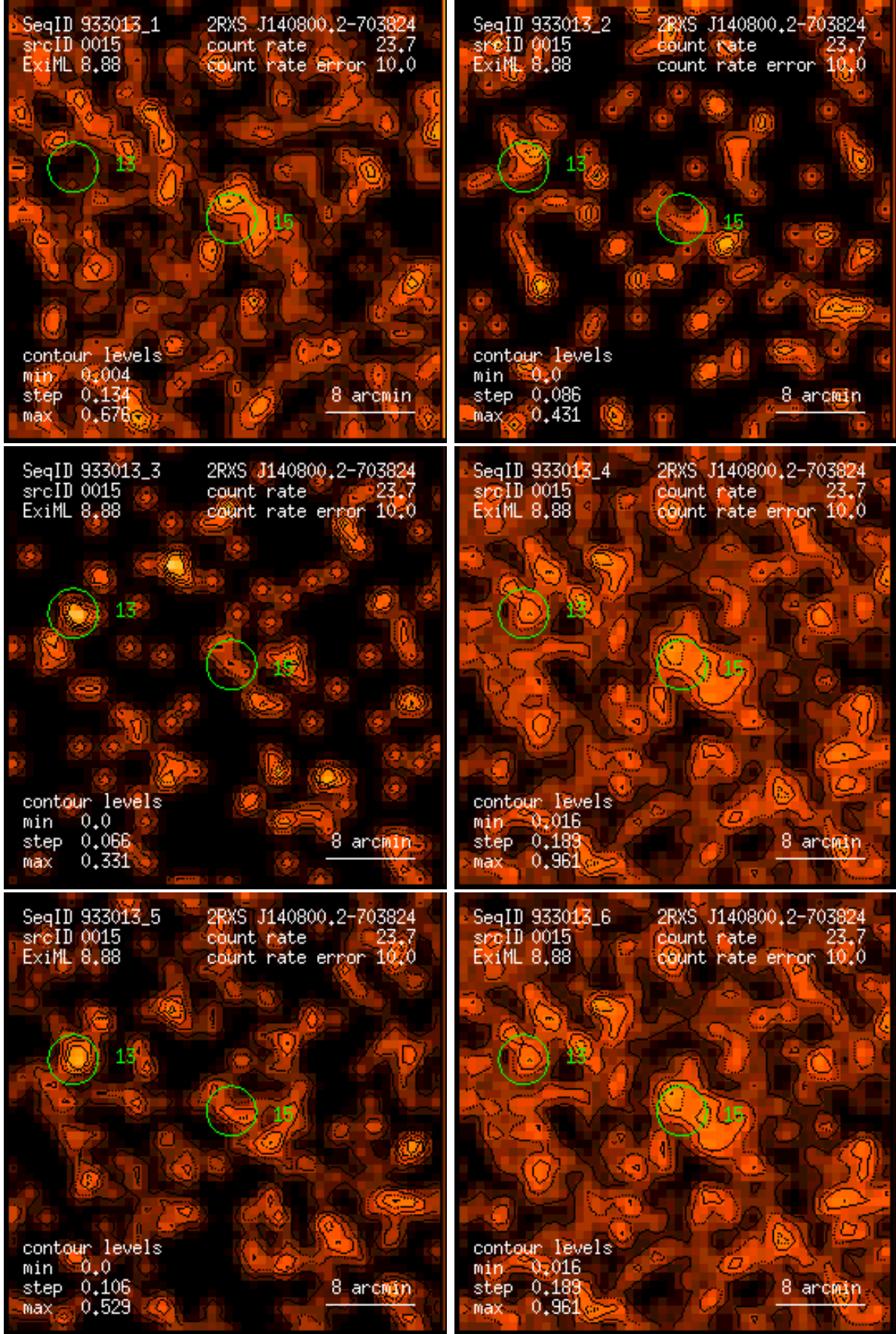
Figure 15: RASS 933013: detection 0015: band rate images, Gaussian filter: (1) PSPC channels 11 – 41, (2) 52 – 90, (3) 91 – 201, (4) 11 – 235, (5) 52 – 201, (6) 11 – 201. Broad band rates in counts/ks. Band rate contour levels in counts/ks/arcmin 2 .
