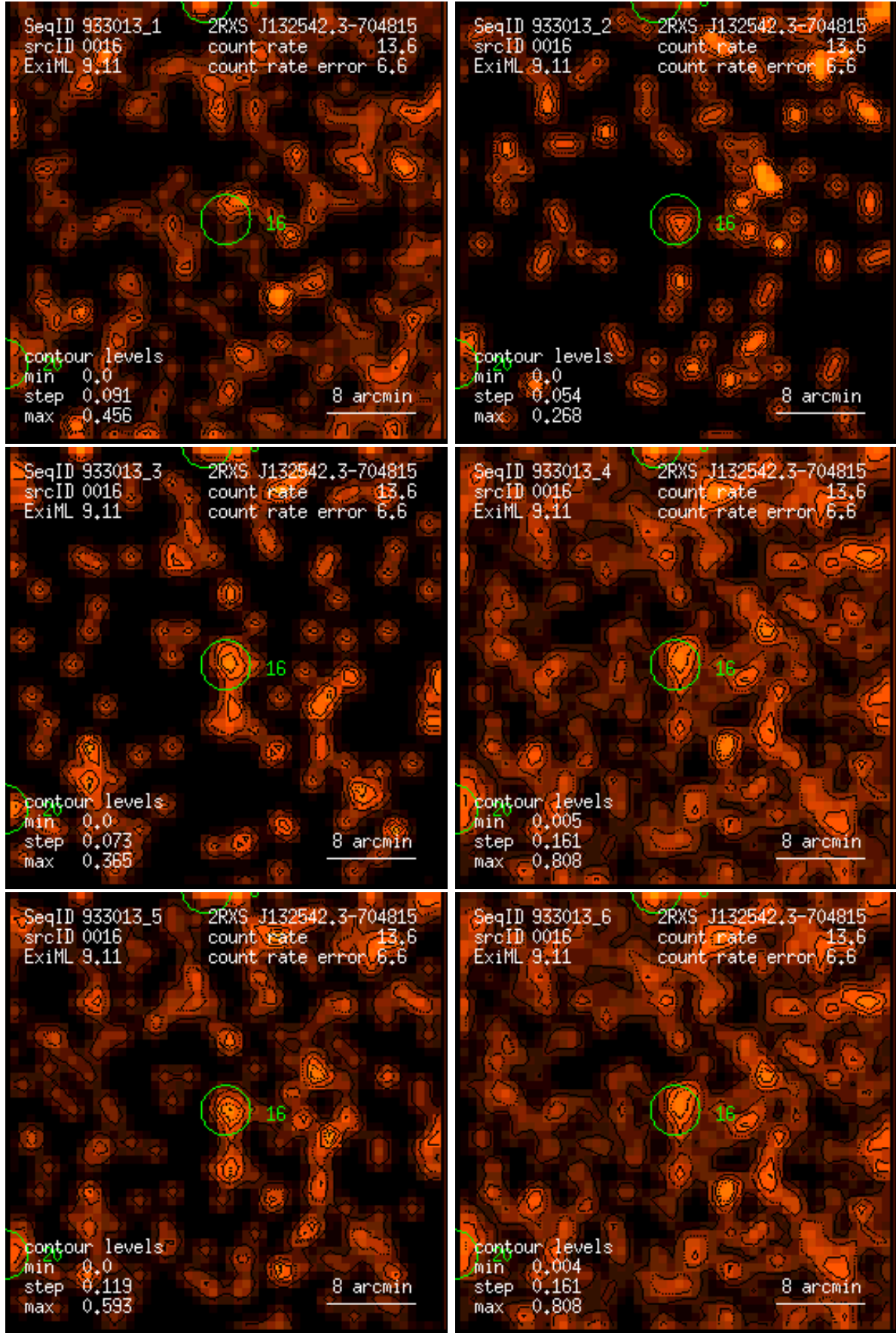
Figure 16: RASS 933013: detection 0016: band rate images, Gaussian filter: (1) PSPC channels 11 – 41, (2) 52 – 90, (3) 91 – 201, (4) 11 – 235, (5) 52 – 201, (6) 11 – 201. Broad band rates in counts/ks. Band rate contour levels in counts/ks/arcmin 2 .
