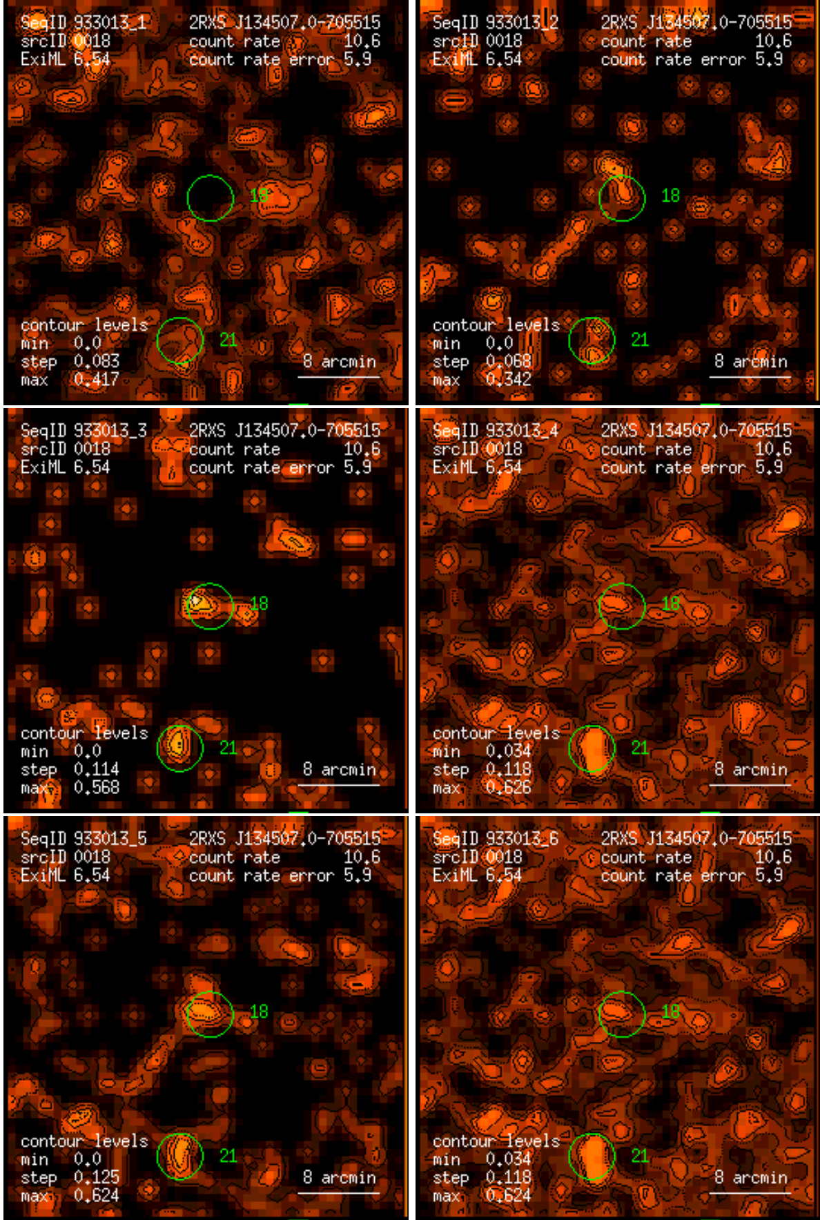
Figure 18: RASS 933013: detection 0018: band rate images, Gaussian filter: (1) PSPC channels 11 – 41, (2) 52 – 90, (3) 91 – 201, (4) 11 – 235, (5) 52 – 201, (6) 11 – 201. Broad band rates in counts/ks. Band rate contour levels in counts/ks/arcmin 2 .
