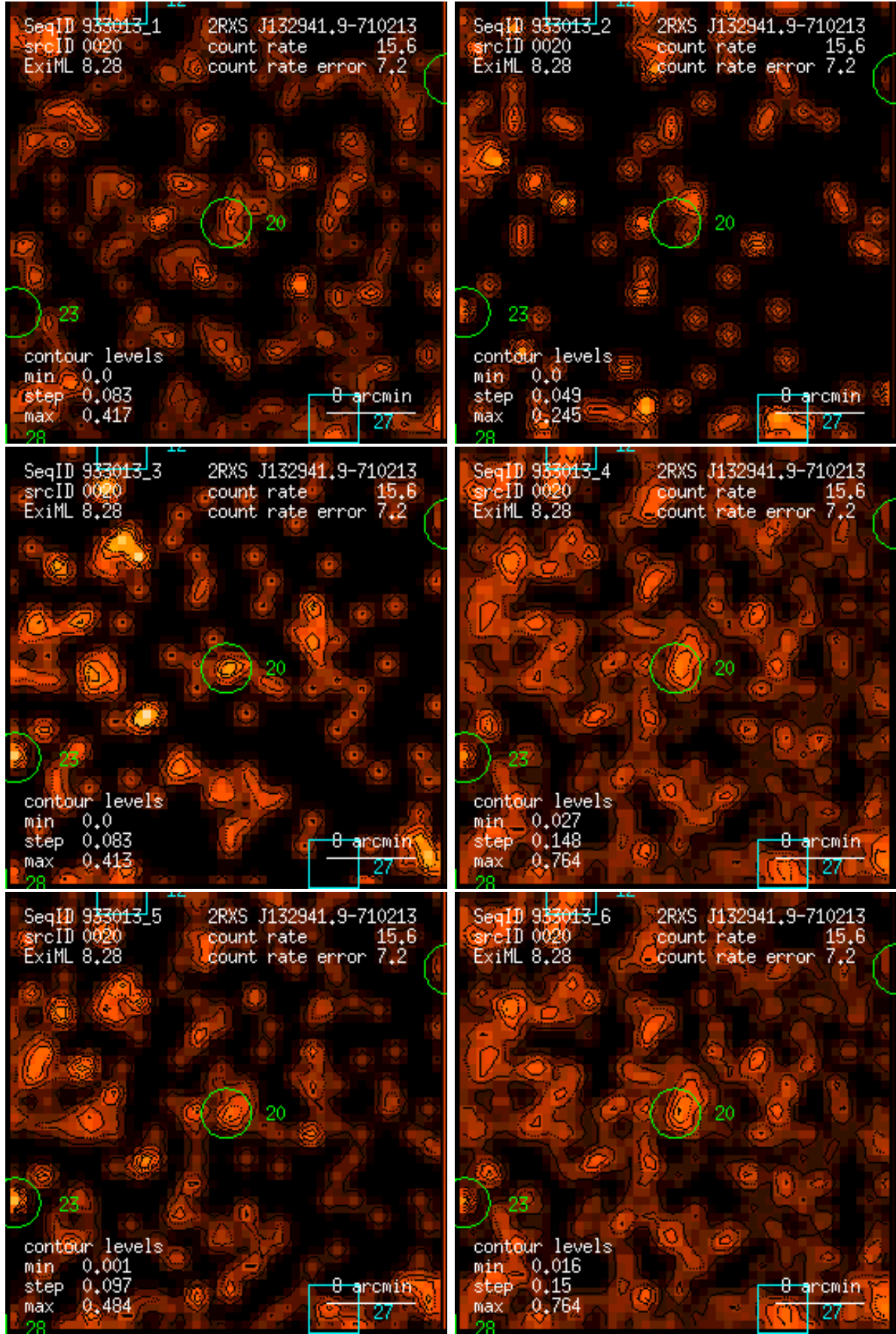
Figure 20: RASS 933013: detection 0020: band rate images, Gaussian filter: (1) PSPC channels 11 – 41, (2) 52 – 90, (3) 91 – 201, (4) 11 – 235, (5) 52 – 201, (6) 11 – 201. Broad band rates in counts/ks. Band rate contour levels in counts/ks/arcmin 2 .
