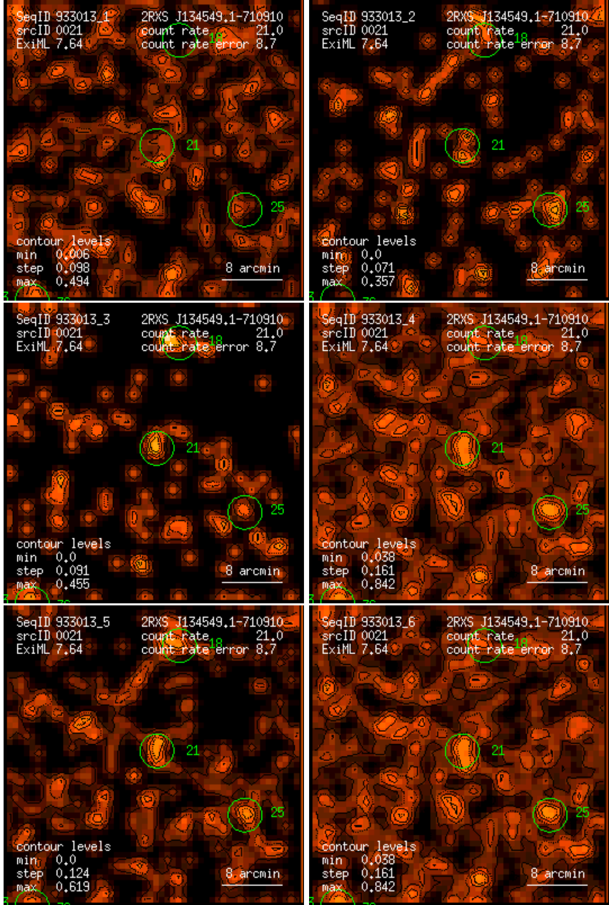
Figure 21: RASS 933013: detection 0021: band rate images, Gaussian filter: (1) PSPC channels 11 – 41, (2) 52 – 90, (3) 91 – 201, (4) 11 – 235, (5) 52 – 201, (6) 11 – 201. Broad band rates in counts/ks. Band rate contour levels in counts/ks/arcmin 2 .
