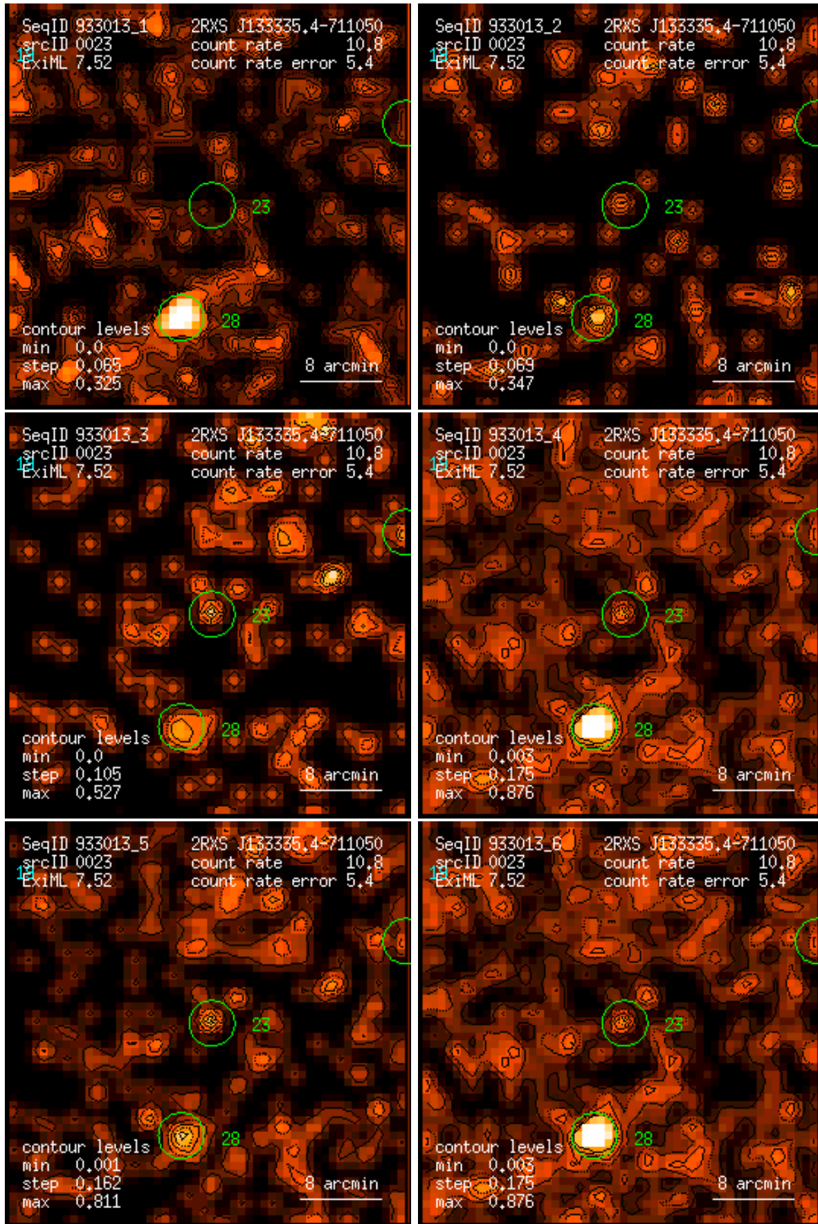
Figure 23: RASS 933013: detection 0023: band rate images, Gaussian filter: (1) PSPC channels 11 – 41, (2) 52 – 90, (3) 91 – 201, (4) 11 – 235, (5) 52 – 201, (6) 11 – 201. Broad band rates in counts/ks. Band rate contour levels in counts/ks/arcmin 2 .
