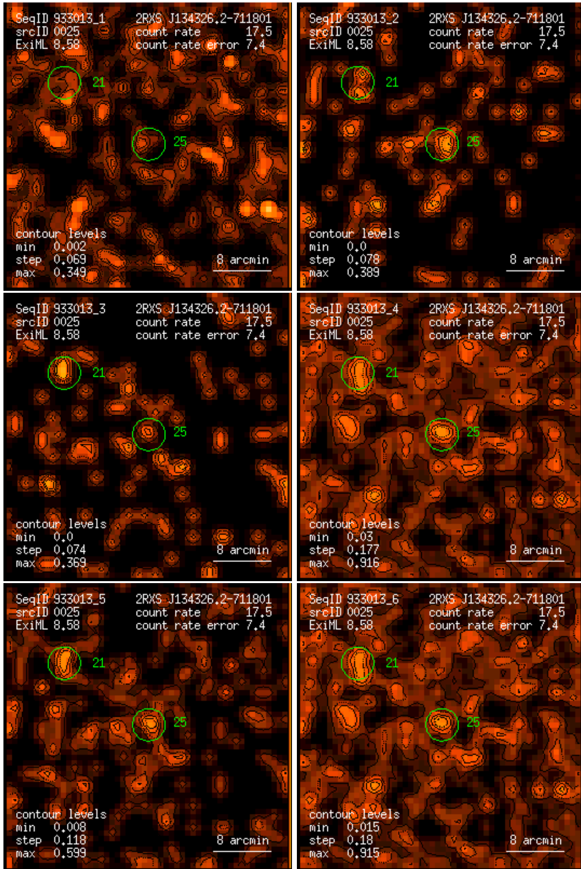
Figure 25: RASS 933013: detection 0025: band rate images, Gaussian filter: (1) PSPC channels 11 – 41, (2) 52 – 90, (3) 91 – 201, (4) 11 – 235, (5) 52 – 201, (6) 11 – 201. Broad band rates in counts/ks. Band rate contour levels in counts/ks/arcmin 2 .
