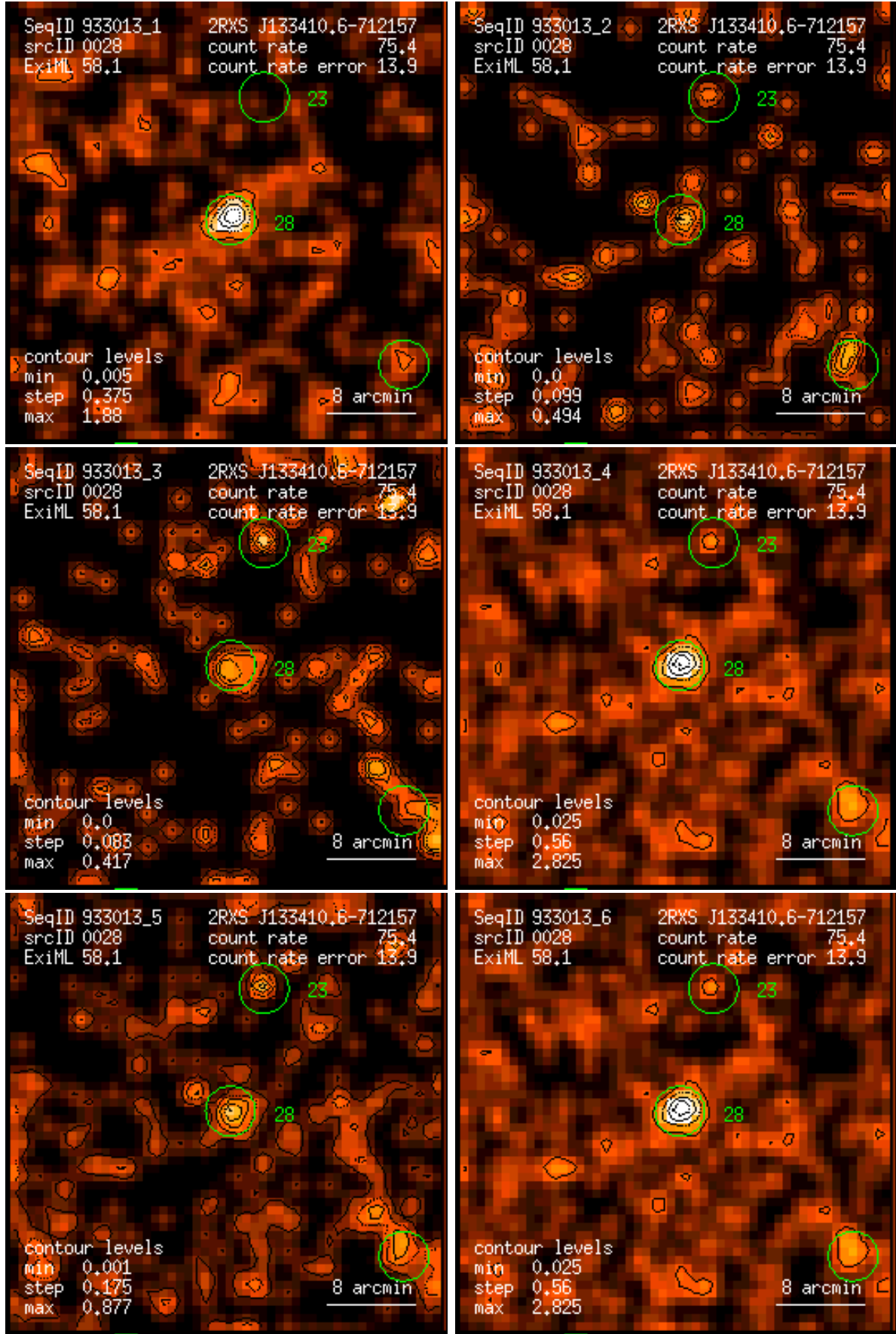
Figure 28: RASS 933013: detection 0028: band rate images, Gaussian filter: (1) PSPC channels 11 – 41, (2) 52 – 90, (3) 91 – 201, (4) 11 – 235, (5) 52 – 201, (6) 11 – 201. Broad band rates in counts/ks. Band rate contour levels in counts/ks/arcmin 2 .
