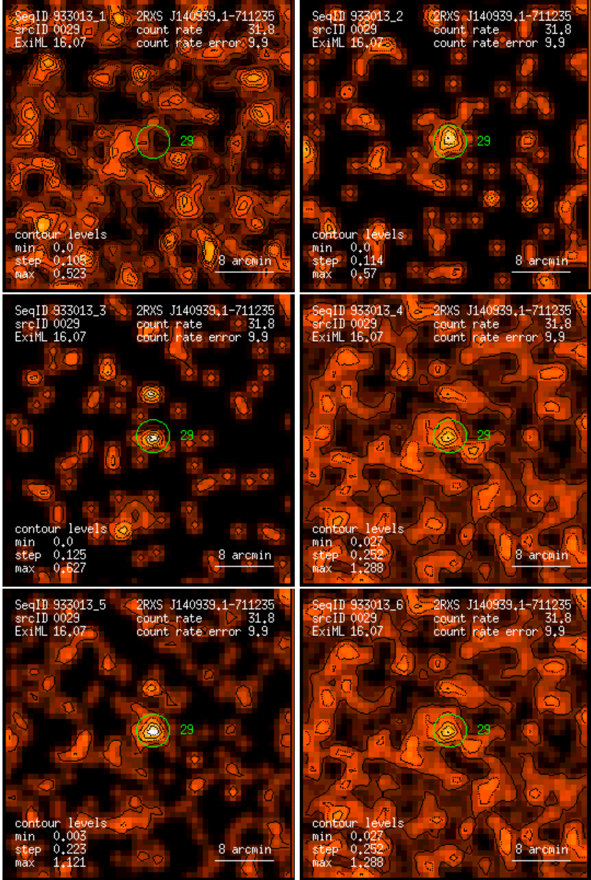
Figure 29: RASS 933013: detection 0029: band rate images, Gaussian filter: (1) PSPC channels 11 – 41, (2) 52 – 90, (3) 91 – 201, (4) 11 – 235, (5) 52 – 201, (6) 11 – 201. Broad band rates in counts/ks. Band rate contour levels in counts/ks/arcmin 2 .
