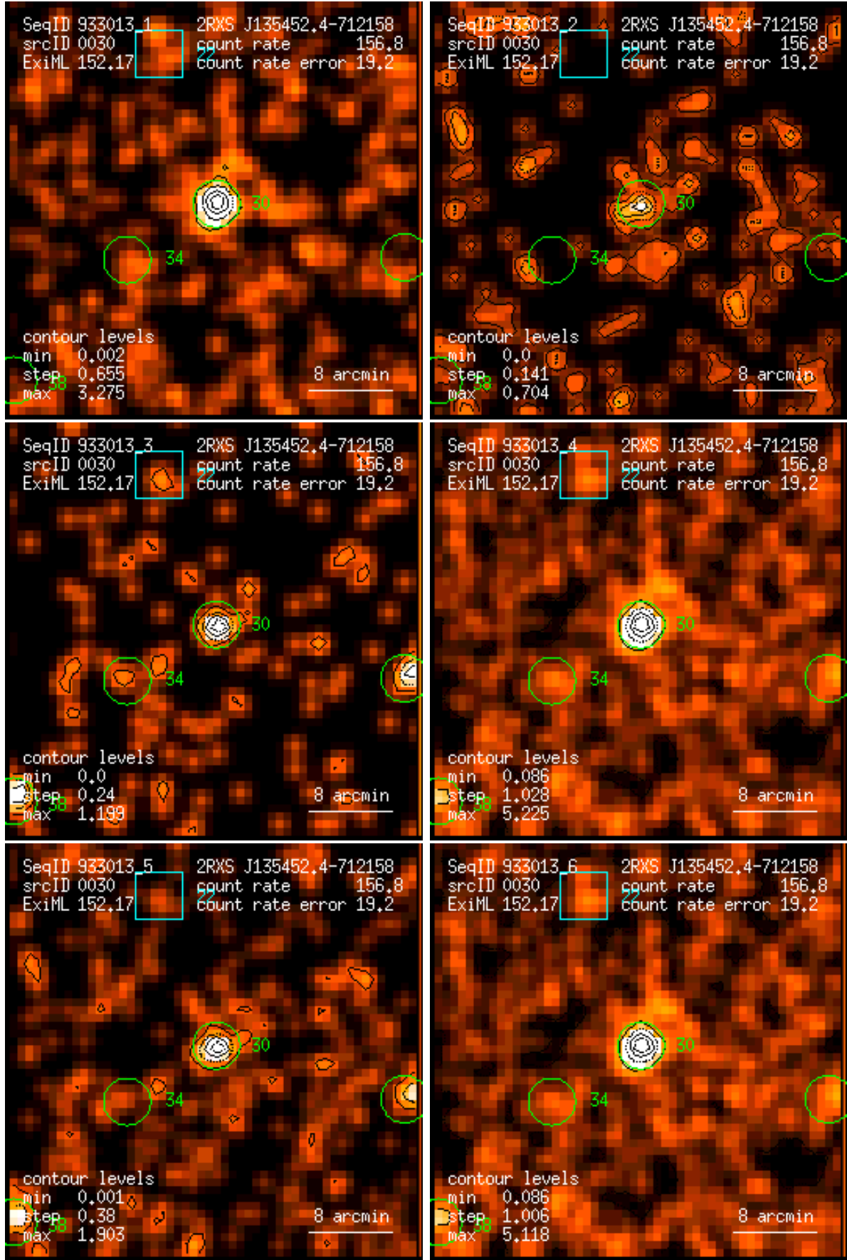
Figure 30: RASS 933013: detection 0030: band rate images, Gaussian filter: (1) PSPC channels 11 – 41, (2) 52 – 90, (3) 91 – 201, (4) 11 – 235, (5) 52 – 201, (6) 11 – 201. Broad band rates in counts/ks. Band rate contour levels in counts/ks/arcmin 2 .
