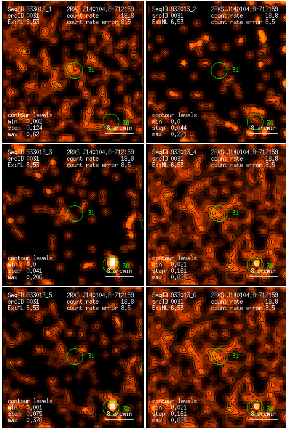
Figure 31: RASS 933013: detection 0031: band rate images, Gaussian filter: (1) PSPC channels 11 – 41, (2) 52 – 90, (3) 91 – 201, (4) 11 – 235, (5) 52 – 201, (6) 11 – 201. Broad band rates in counts/ks. Band rate contour levels in counts/ks/arcmin 2 .
