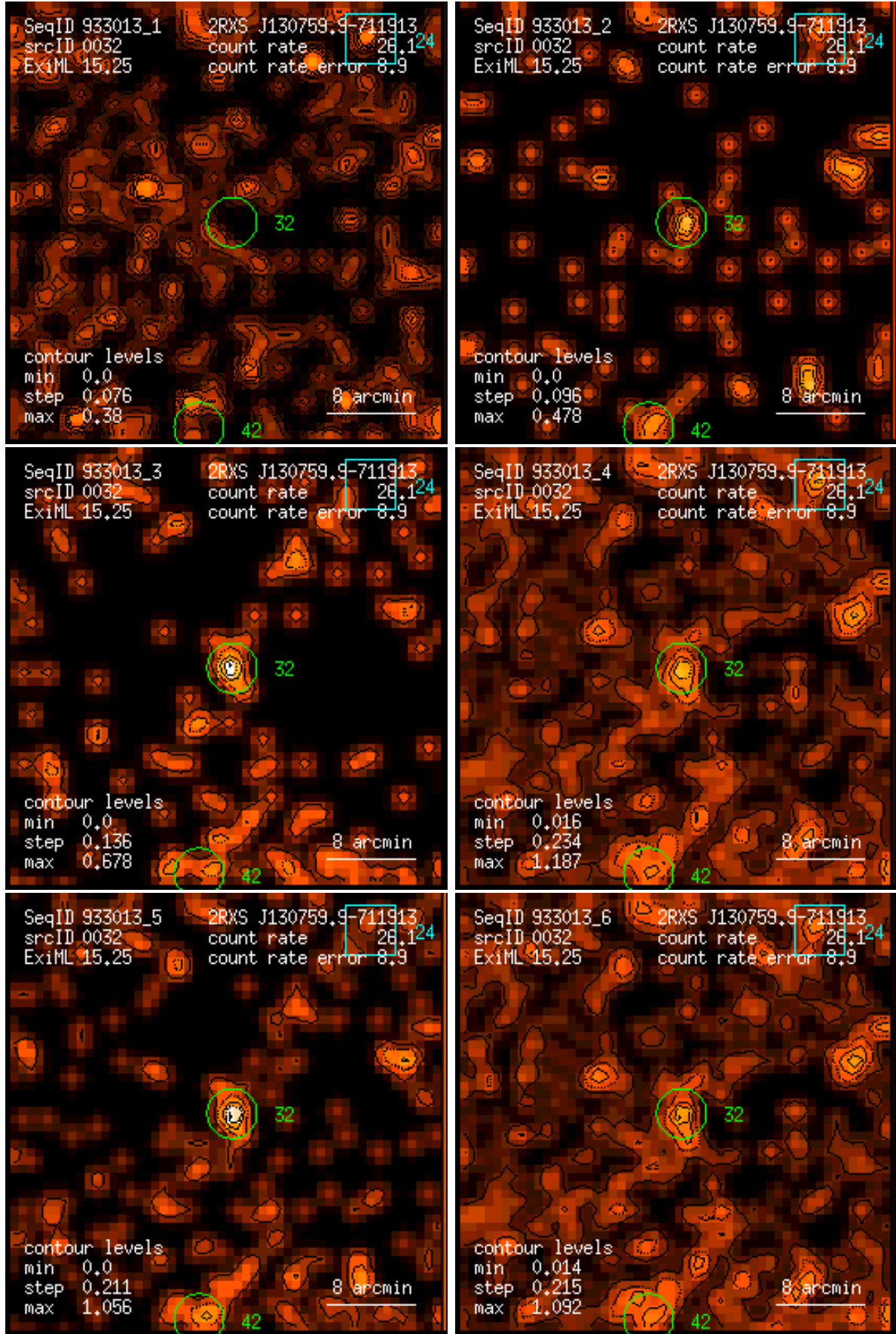
Figure 32: RASS 933013: detection 0032: band rate images, Gaussian filter: (1) PSPC channels 11 – 41, (2) 52 – 90, (3) 91 – 201, (4) 11 – 235, (5) 52 – 201, (6) 11 – 201. Broad band rates in counts/ks. Band rate contour levels in counts/ks/arcmin 2 .
