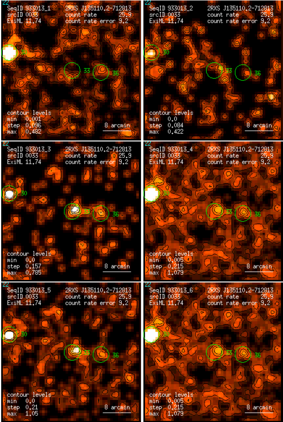
Figure 33: RASS 933013: detection 0033: band rate images, Gaussian filter: (1) PSPC channels 11 – 41, (2) 52 – 90, (3) 91 – 201, (4) 11 – 235, (5) 52 – 201, (6) 11 – 201. Broad band rates in counts/ks. Band rate contour levels in counts/ks/arcmin 2 .
