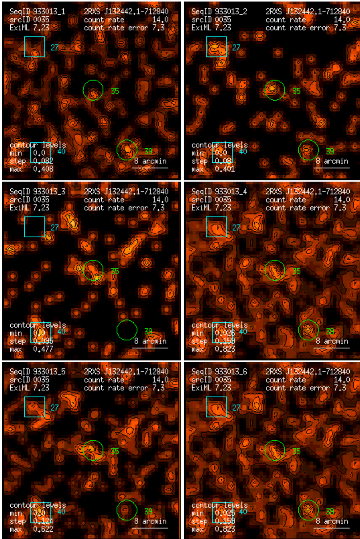
Figure 35: RASS 933013: detection 0035: band rate images, Gaussian filter: (1) PSPC channels 11 – 41, (2) 52 – 90, (3) 91 – 201, (4) 11 – 235, (5) 52 – 201, (6) 11 – 201. Broad band rates in counts/ks. Band rate contour levels in counts/ks/arcmin 2 .
