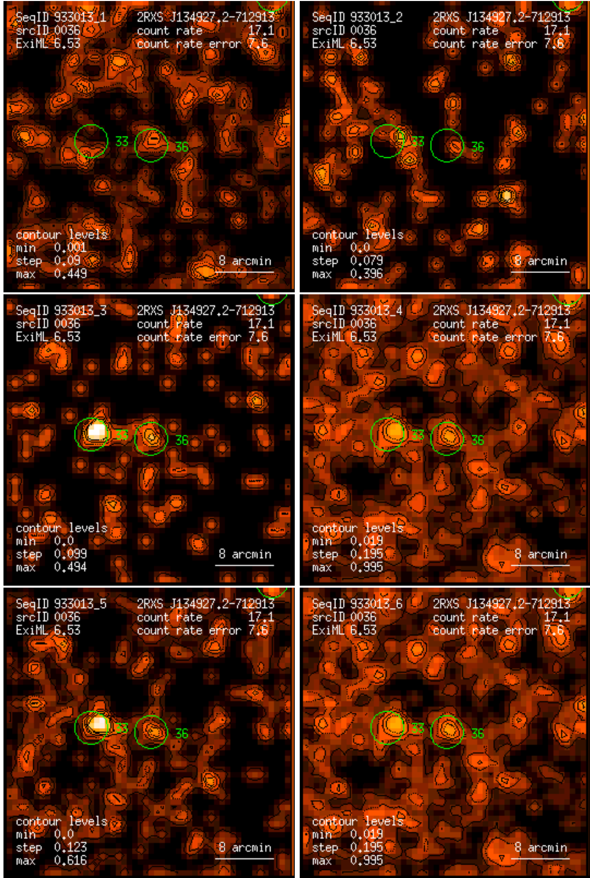
Figure 36: RASS 933013: detection 0036: band rate images, Gaussian filter: (1) PSPC channels 11 – 41, (2) 52 – 90, (3) 91 – 201, (4) 11 – 235, (5) 52 – 201, (6) 11 – 201. Broad band rates in counts/ks. Band rate contour levels in counts/ks/arcmin 2 .
