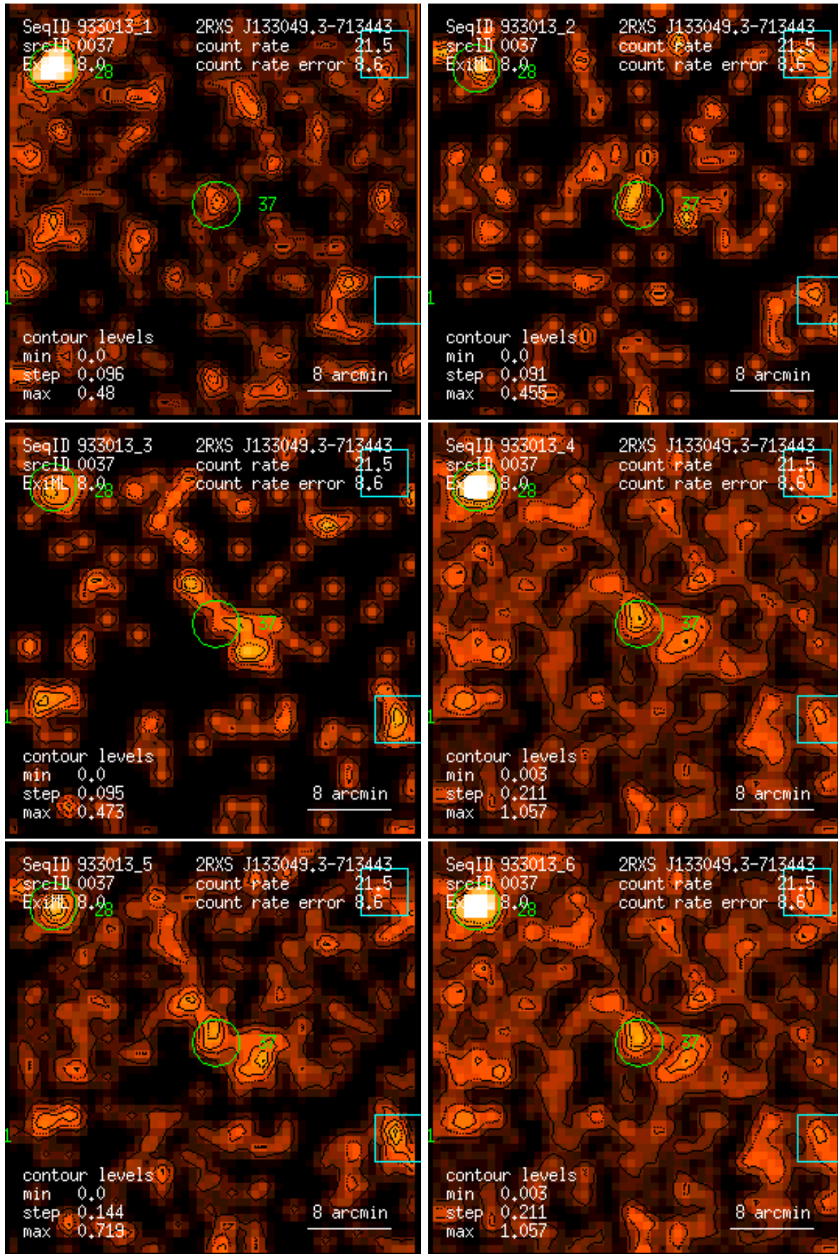
Figure 37: RASS 933013: detection 0037: band rate images, Gaussian filter: (1) PSPC channels 11 – 41, (2) 52 – 90, (3) 91 – 201, (4) 11 – 235, (5) 52 – 201, (6) 11 – 201. Broad band rates in counts/ks. Band rate contour levels in counts/ks/arcmin 2 .
