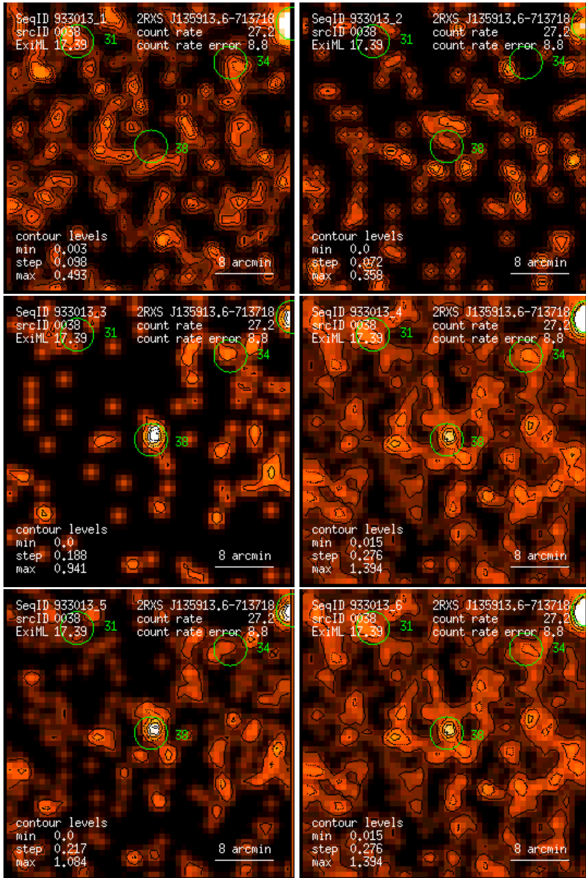
Figure 38: RASS 933013: detection 0038: band rate images, Gaussian filter: (1) PSPC channels 11 – 41, (2) 52 – 90, (3) 91 – 201, (4) 11 – 235, (5) 52 – 201, (6) 11 – 201. Broad band rates in counts/ks. Band rate contour levels in counts/ks/arcmin 2 .
