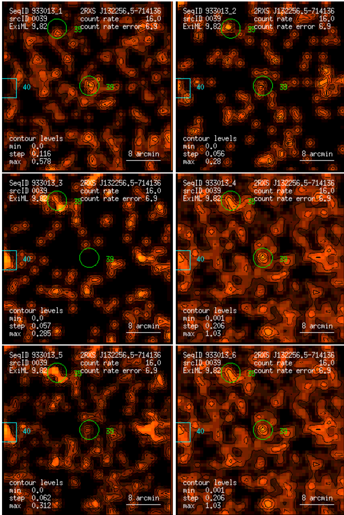
Figure 39: RASS 933013: detection 0039: band rate images, Gaussian filter: (1) PSPC channels 11 – 41, (2) 52 – 90, (3) 91 – 201, (4) 11 – 235, (5) 52 – 201, (6) 11 – 201. Broad band rates in counts/ks. Band rate contour levels in counts/ks/arcmin 2 .
