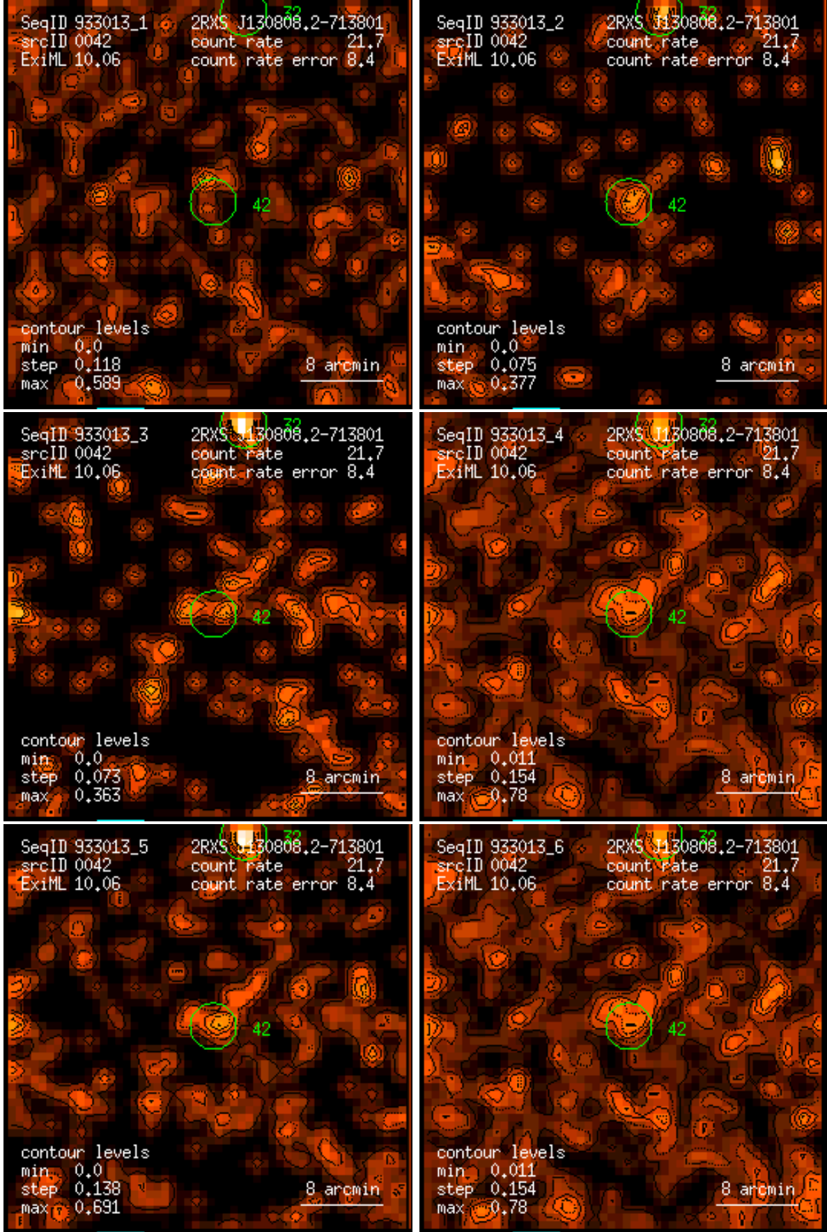
Figure 42: RASS 933013: detection 0042: band rate images, Gaussian filter: (1) PSPC channels 11 – 41, (2) 52 – 90, (3) 91 – 201, (4) 11 – 235, (5) 52 – 201, (6) 11 – 201. Broad band rates in counts/ks. Band rate contour levels in counts/ks/arcmin 2 .
