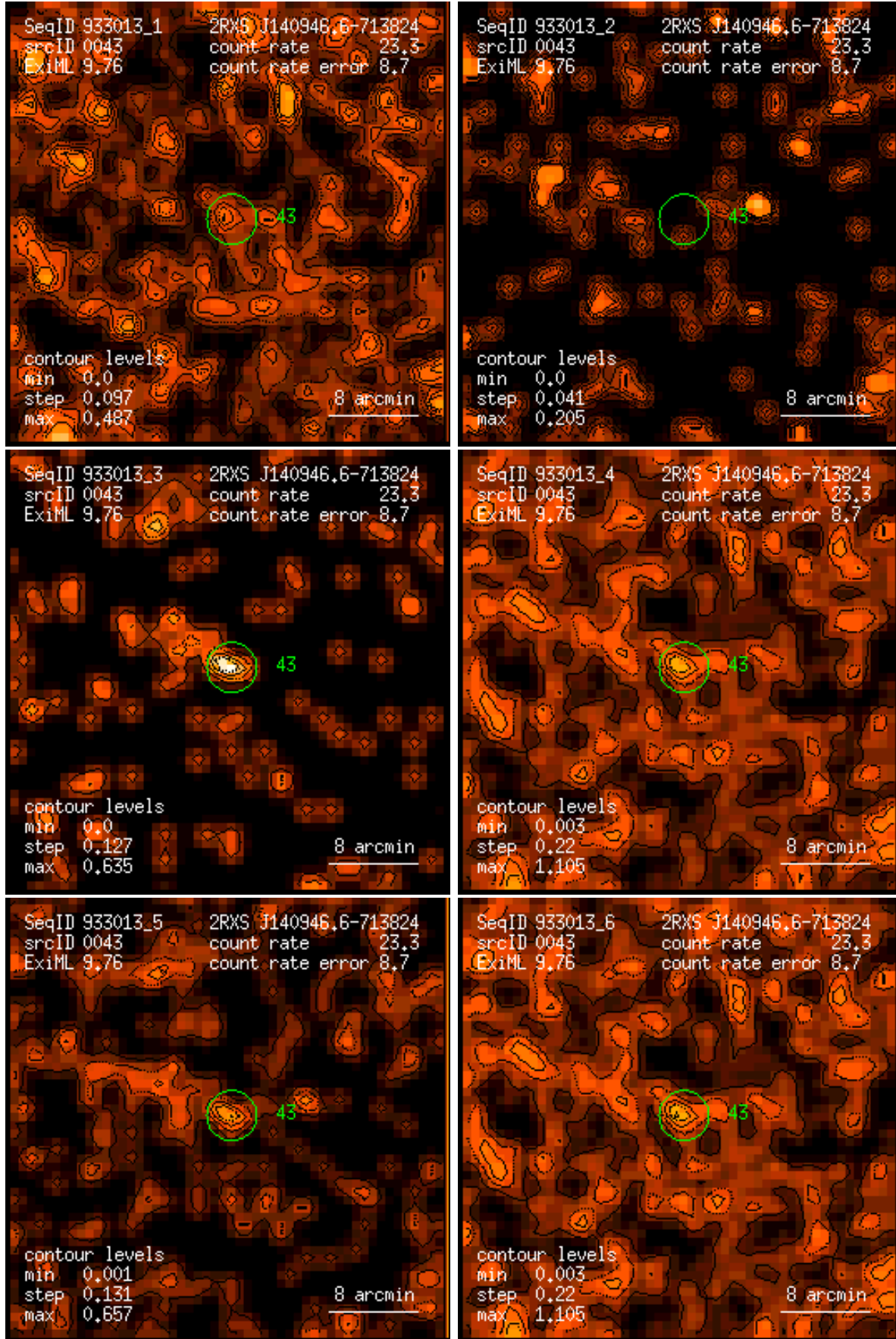
Figure 43: RASS 933013: detection 0043: band rate images, Gaussian filter: (1) PSPC channels 11 – 41, (2) 52 – 90, (3) 91 – 201, (4) 11 – 235, (5) 52 – 201, (6) 11 – 201. Broad band rates in counts/ks. Band rate contour levels in counts/ks/arcmin 2 .
