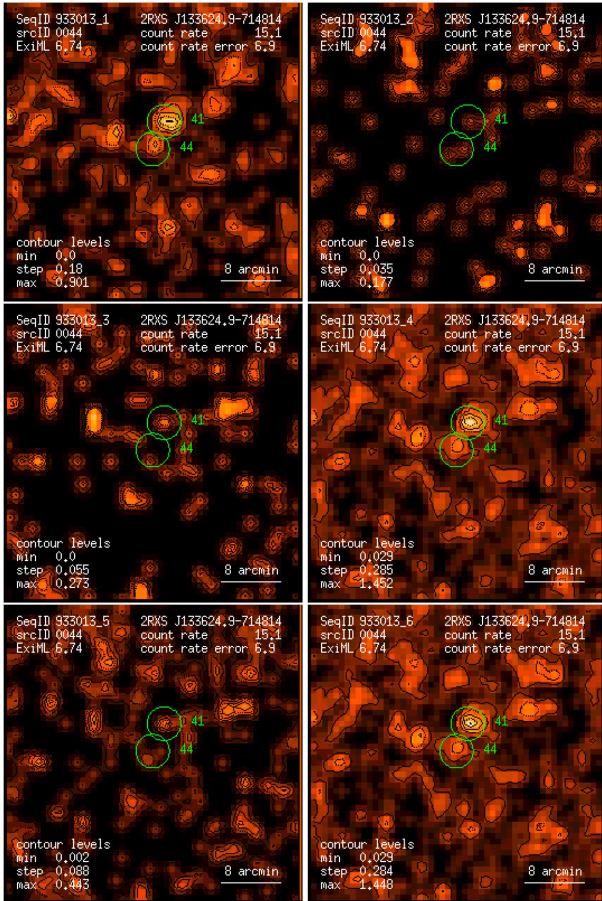
Figure 44: RASS 933013: detection 0044: band rate images, Gaussian filter: (1) PSPC channels 11 – 41, (2) 52 – 90, (3) 91 – 201, (4) 11 – 235, (5) 52 – 201, (6) 11 – 201. Broad band rates in counts/ks. Band rate contour levels in counts/ks/arcmin 2 .
