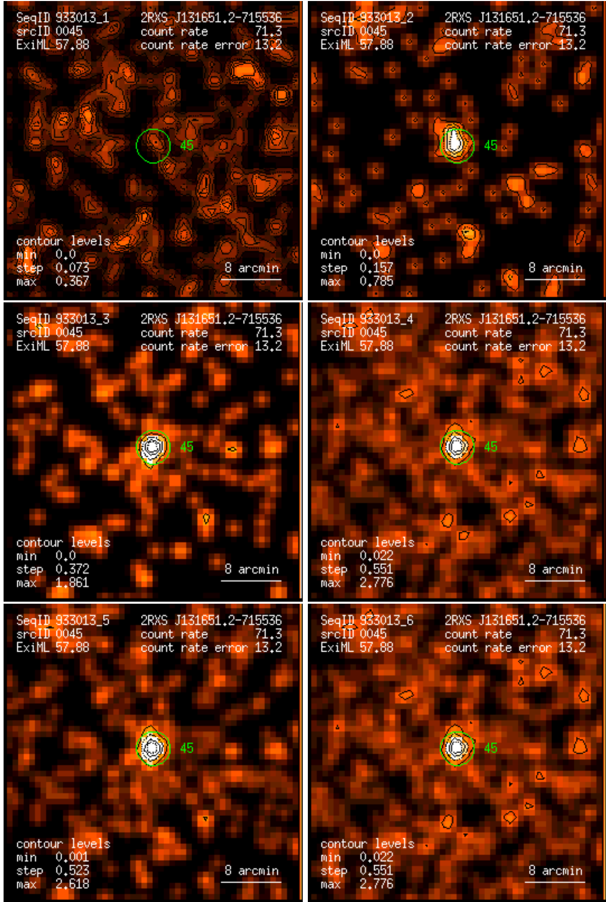
Figure 45: RASS 933013: detection 0045: band rate images, Gaussian filter: (1) PSPC channels 11 – 41, (2) 52 – 90, (3) 91 – 201, (4) 11 – 235, (5) 52 – 201, (6) 11 – 201. Broad band rates in counts/ks. Band rate contour levels in counts/ks/arcmin 2 .
