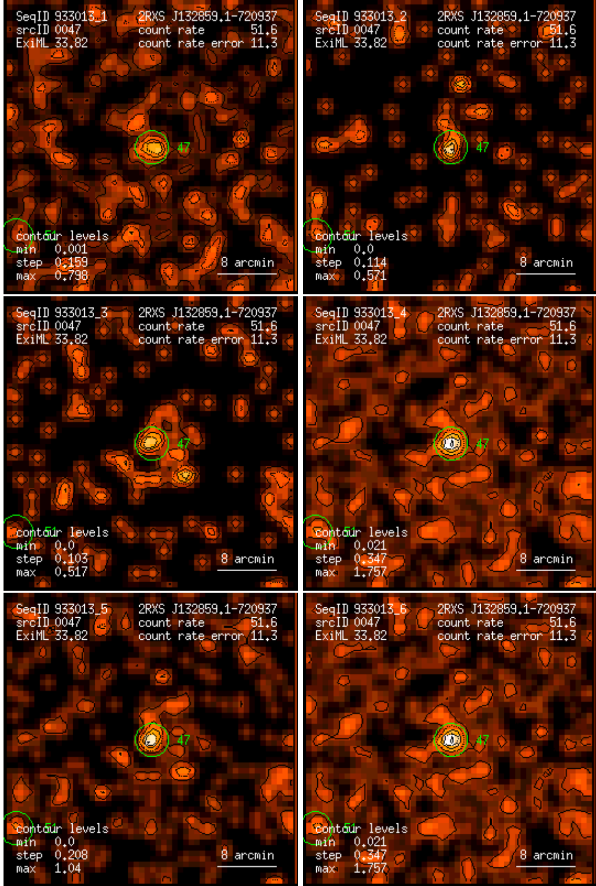
Figure 47: RASS 933013: detection 0047: band rate images, Gaussian filter: (1) PSPC channels 11 – 41, (2) 52 – 90, (3) 91 – 201, (4) 11 – 235, (5) 52 – 201, (6) 11 – 201. Broad band rates in counts/ks. Band rate contour levels in counts/ks/arcmin 2 .
