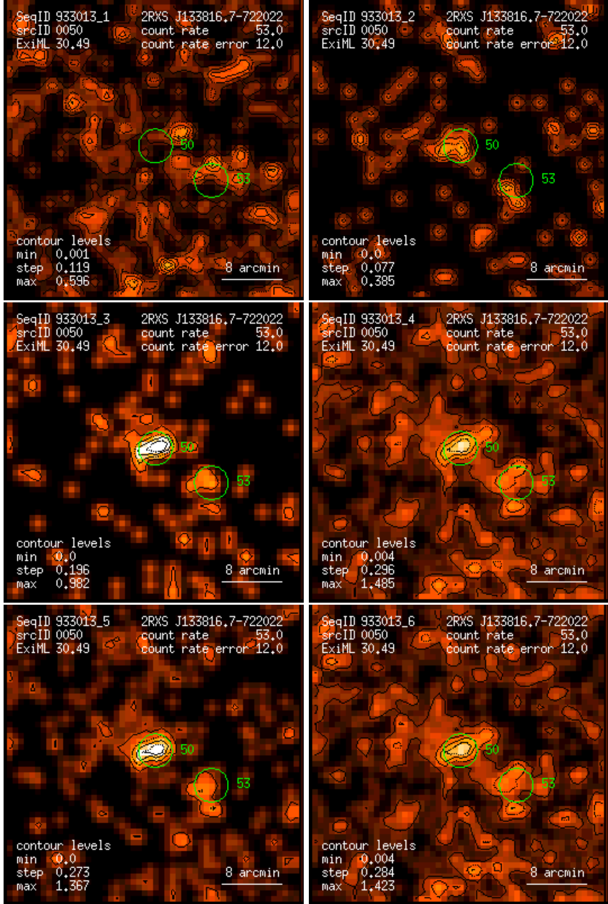
Figure 50: RASS 933013: detection 0050: band rate images, Gaussian filter: (1) PSPC channels 11 – 41, (2) 52 – 90, (3) 91 – 201, (4) 11 – 235, (5) 52 – 201, (6) 11 – 201. Broad band rates in counts/ks. Band rate contour levels in counts/ks/arcmin 2 .
