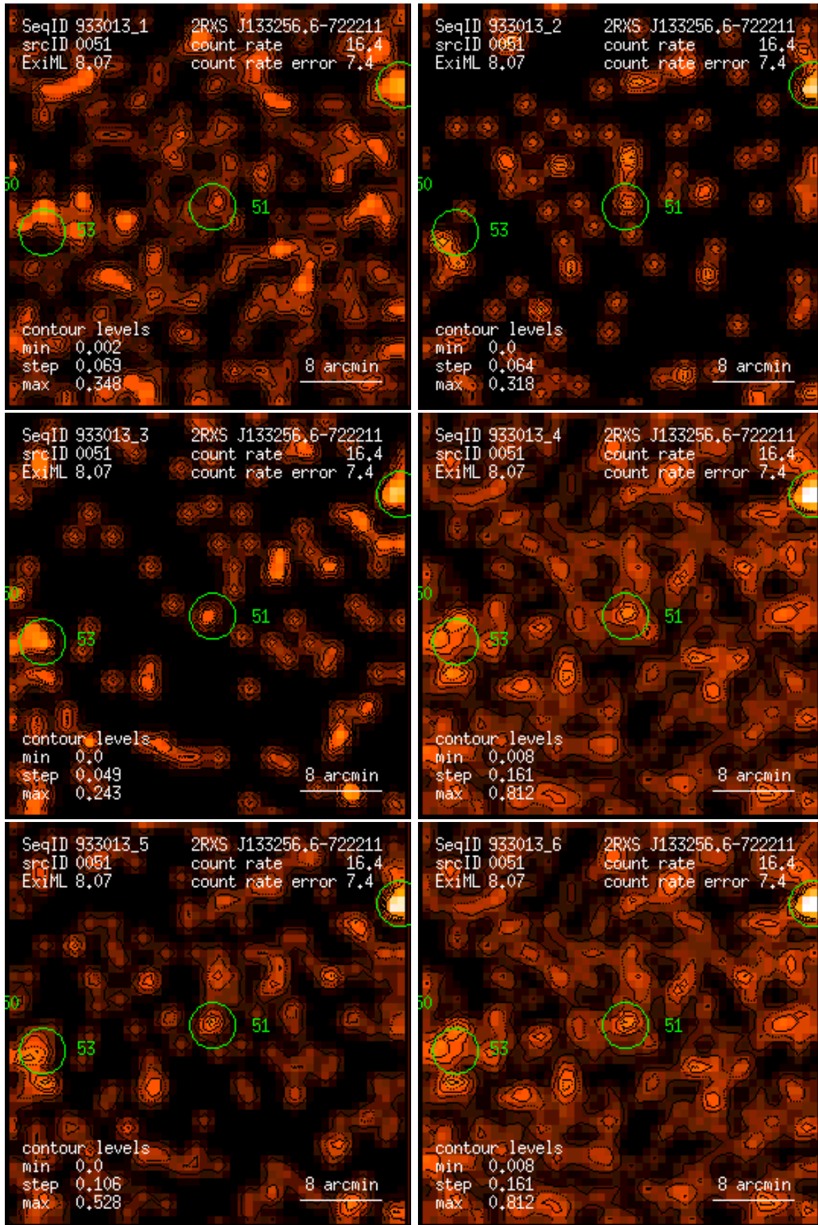
Figure 51: RASS 933013: detection 0051: band rate images, Gaussian filter: (1) PSPC channels 11 – 41, (2) 52 – 90, (3) 91 – 201, (4) 11 – 235, (5) 52 – 201, (6) 11 – 201. Broad band rates in counts/ks. Band rate contour levels in counts/ks/arcmin 2 .
