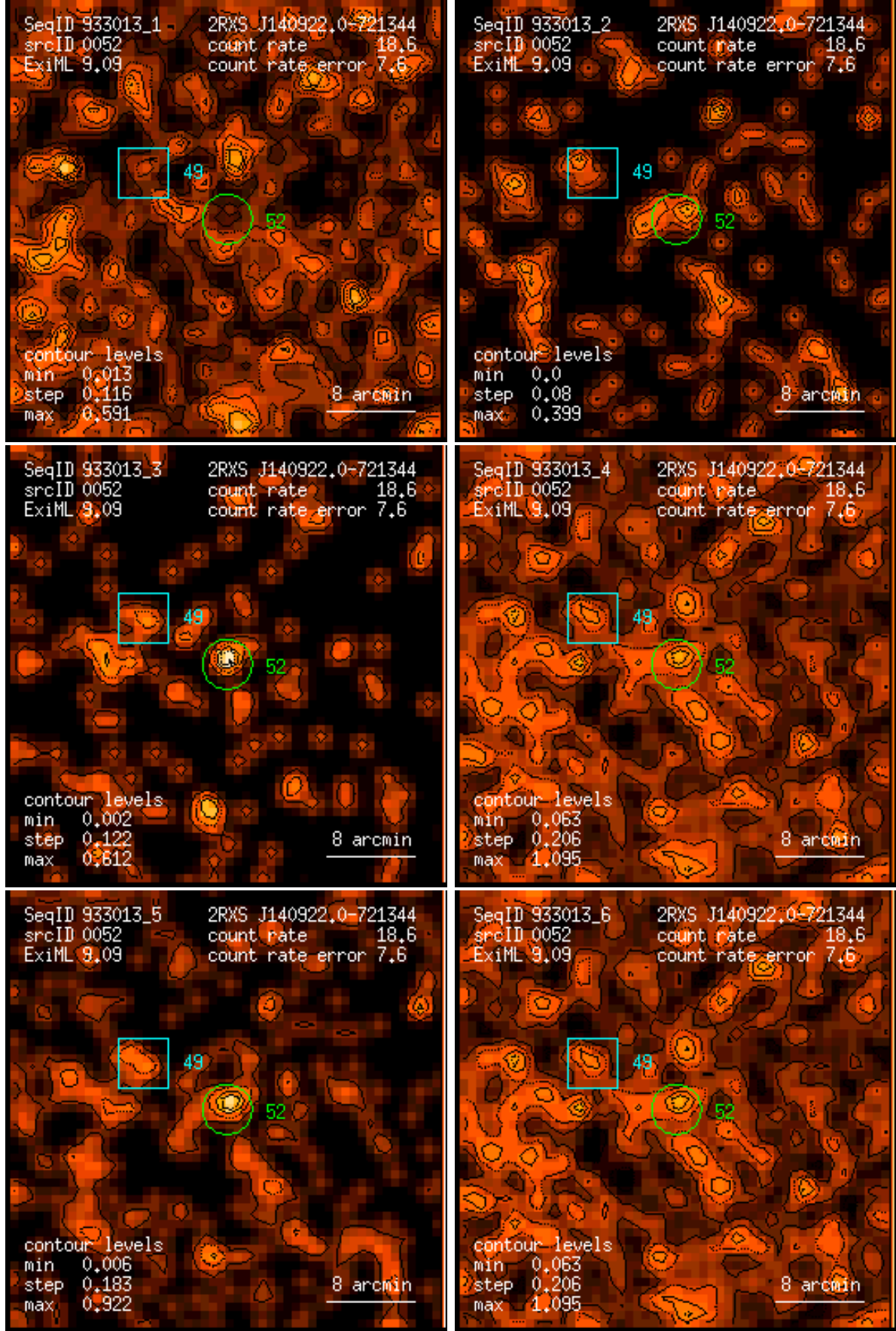
Figure 52: RASS 933013: detection 0052: band rate images, Gaussian filter: (1) PSPC channels 11 – 41, (2) 52 – 90, (3) 91 – 201, (4) 11 – 235, (5) 52 – 201, (6) 11 – 201. Broad band rates in counts/ks. Band rate contour levels in counts/ks/arcmin 2 .
