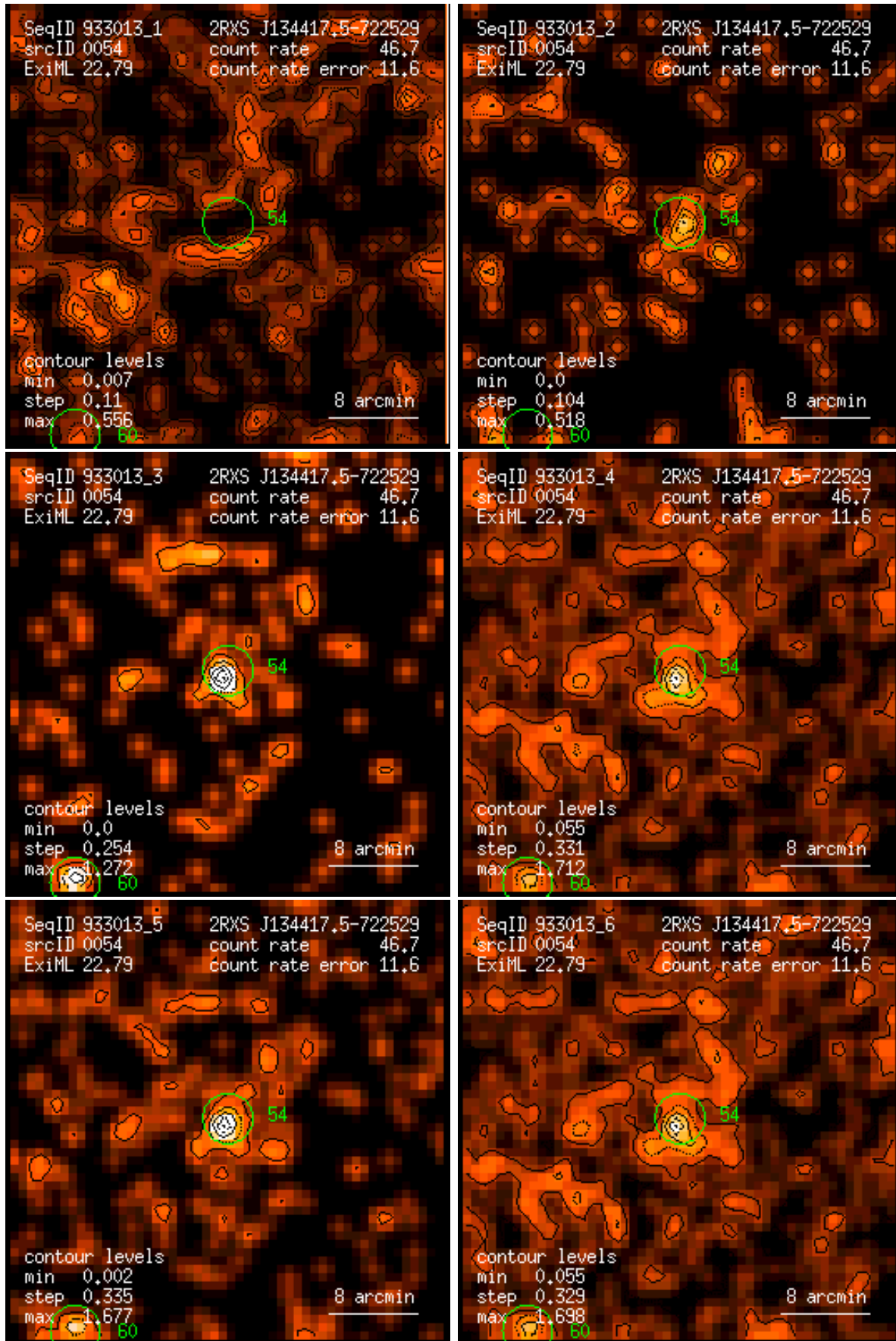
Figure 54: RASS 933013: detection 0054: band rate images, Gaussian filter: (1) PSPC channels 11 – 41, (2) 52 – 90, (3) 91 – 201, (4) 11 – 235, (5) 52 – 201, (6) 11 – 201. Broad band rates in counts/ks. Band rate contour levels in counts/ks/arcmin 2 .
