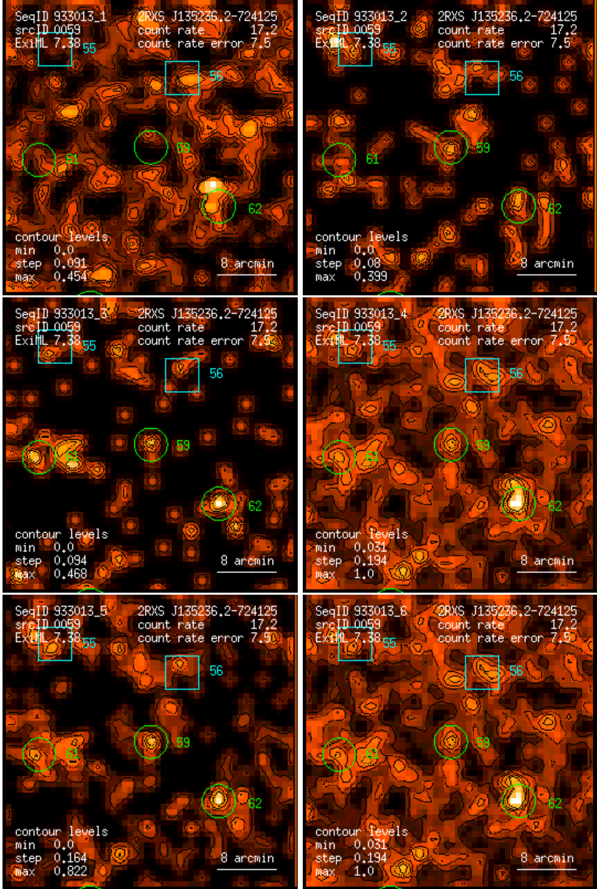
Figure 59: RASS 933013: detection 0059: band rate images, Gaussian filter: (1) PSPC channels 11 – 41, (2) 52 – 90, (3) 91 – 201, (4) 11 – 235, (5) 52 – 201, (6) 11 – 201. Broad band rates in counts/ks. Band rate contour levels in counts/ks/arcmin 2 .
