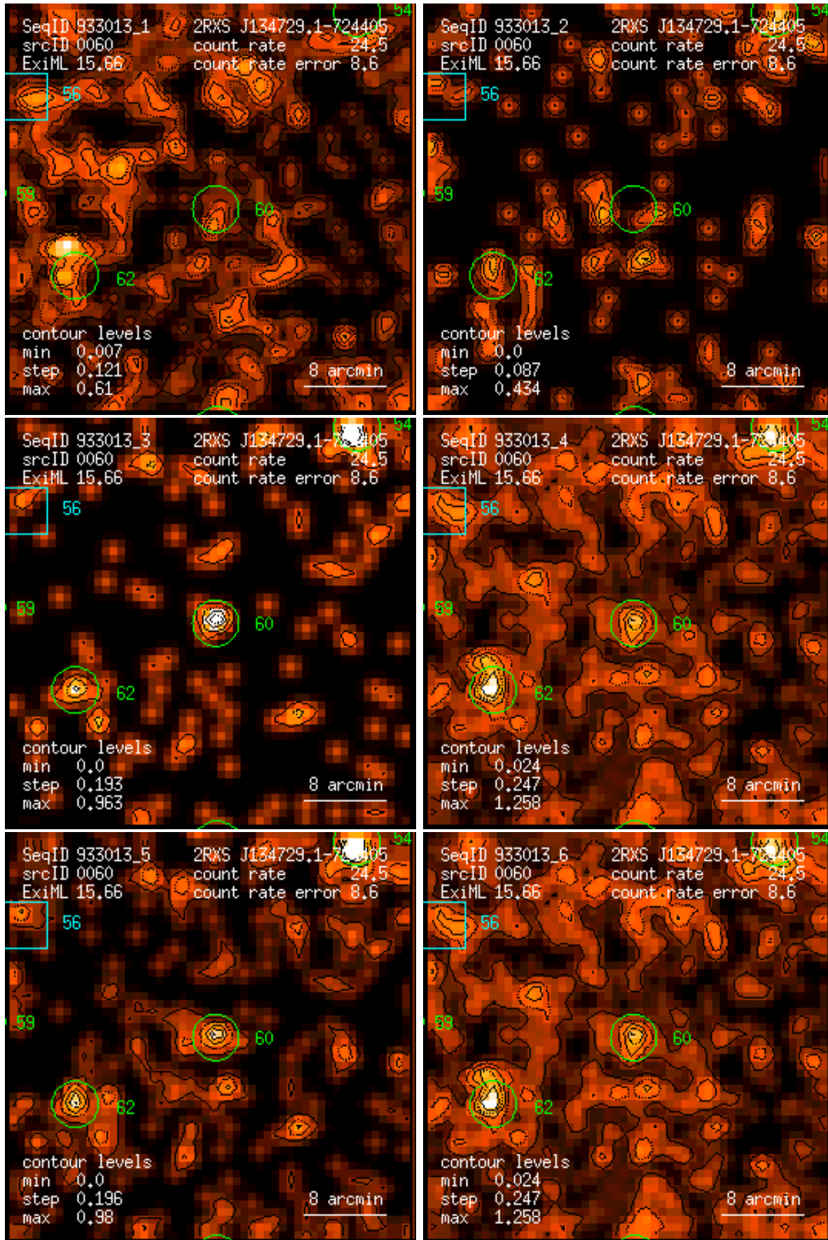
Figure 60: RASS 933013: detection 0060: band rate images, Gaussian filter: (1) PSPC channels 11 – 41, (2) 52 – 90, (3) 91 – 201, (4) 11 – 235, (5) 52 – 201, (6) 11 – 201. Broad band rates in counts/ks. Band rate contour levels in counts/ks/arcmin 2 .
