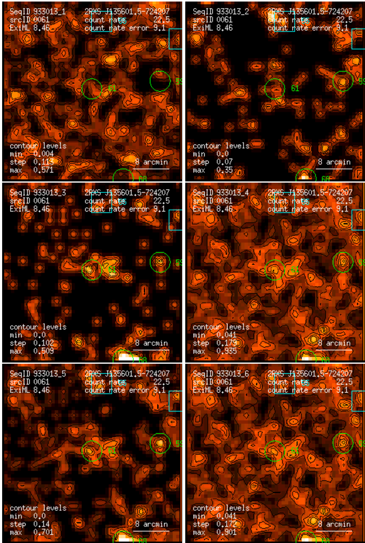
Figure 61: RASS 933013: detection 0061: band rate images, Gaussian filter: (1) PSPC channels 11 – 41, (2) 52 – 90, (3) 91 – 201, (4) 11 – 235, (5) 52 – 201, (6) 11 – 201. Broad band rates in counts/ks. Band rate contour levels in counts/ks/arcmin 2 .
